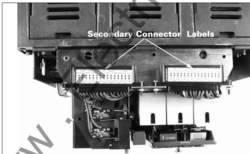
Top View Secondary Connectors Charged
