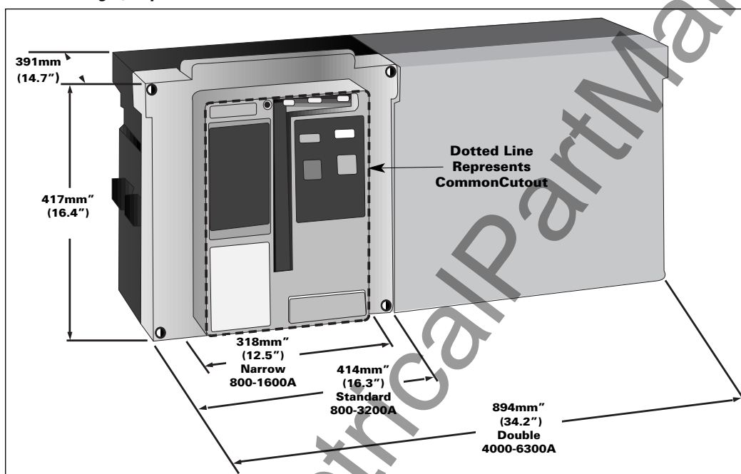
Common Height, Depth and Cutout (3-Pole Illustration)
