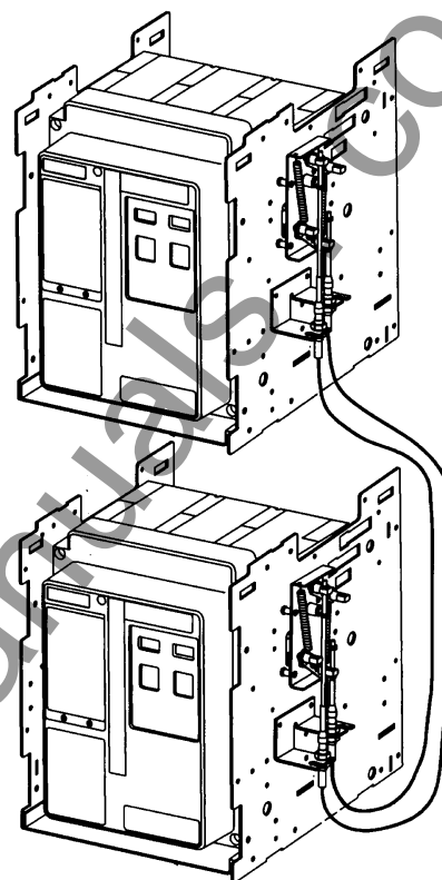
Cassette-Mounted 2-Way Cable Interlock
