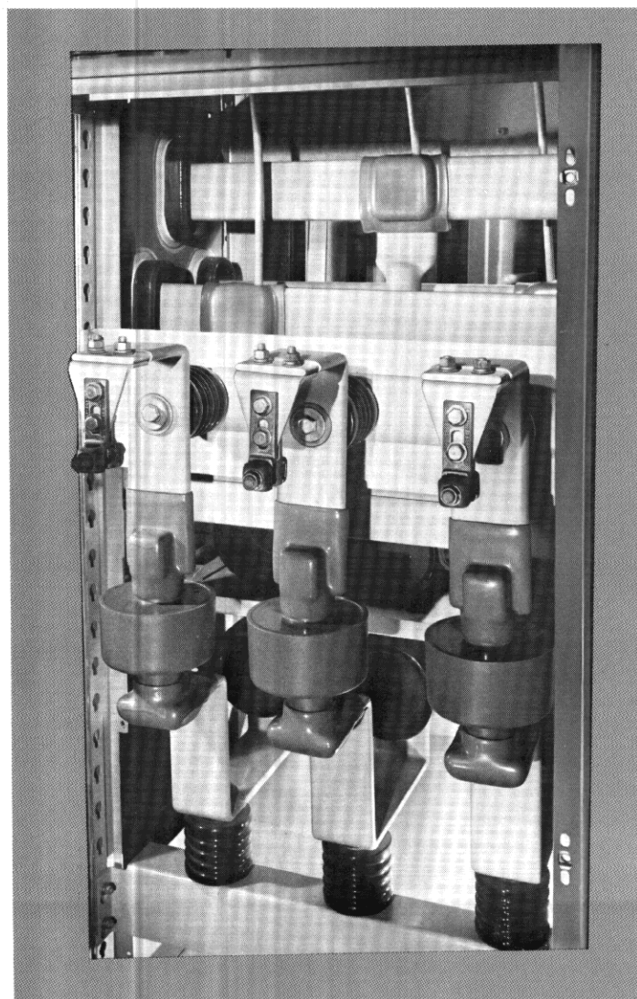
Porcelain bus supports
