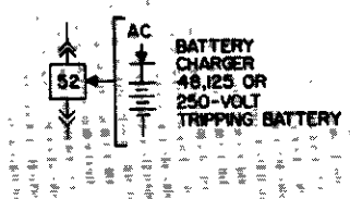
FIG. 3. D-C stored-energy close
