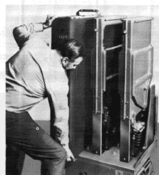
Removing the interphase barriers.
