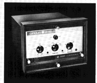
Type ITE-25V Synchronism Check Relay
