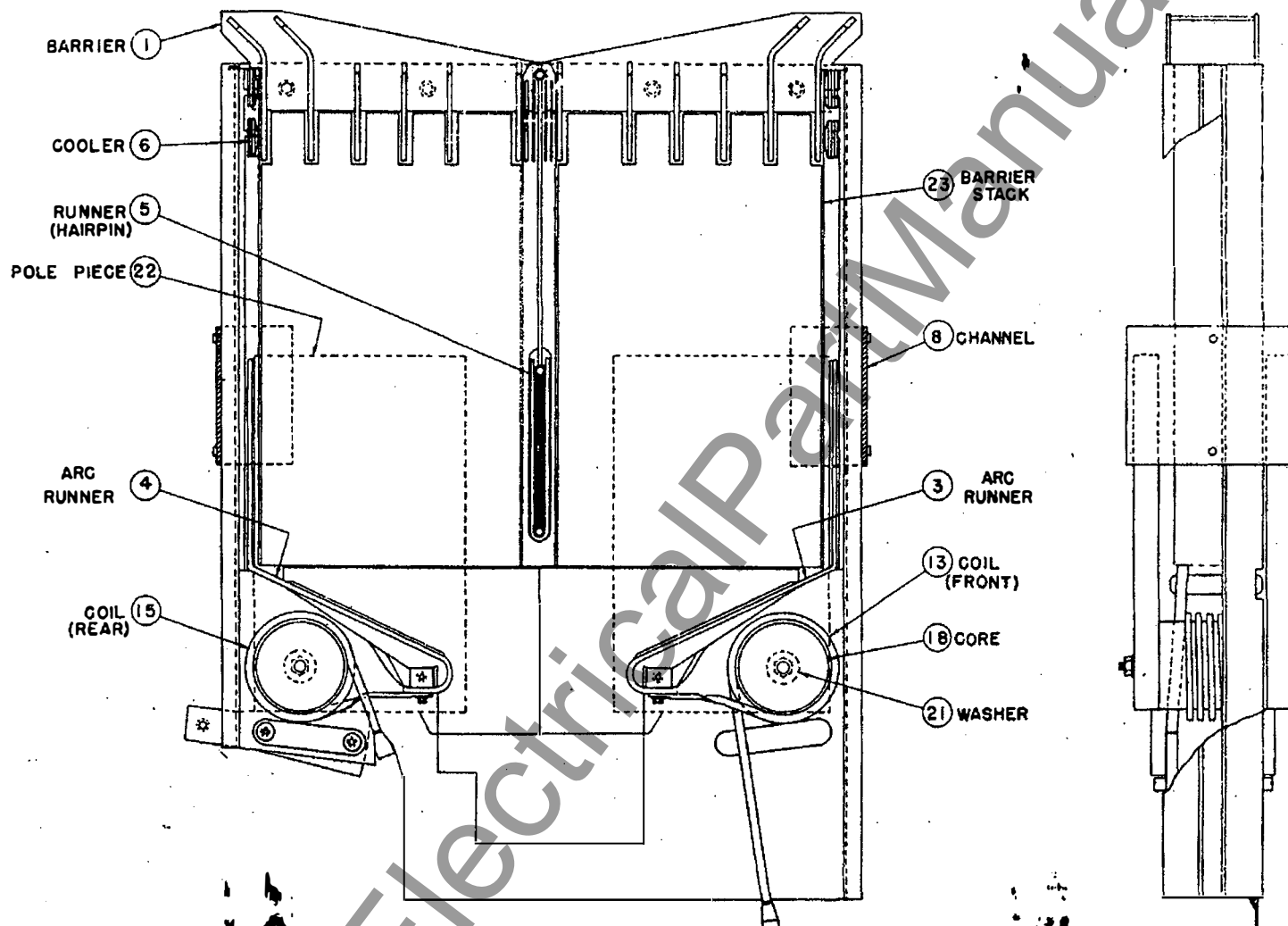
FIG.2 TYPICAL ARC CHUTE
