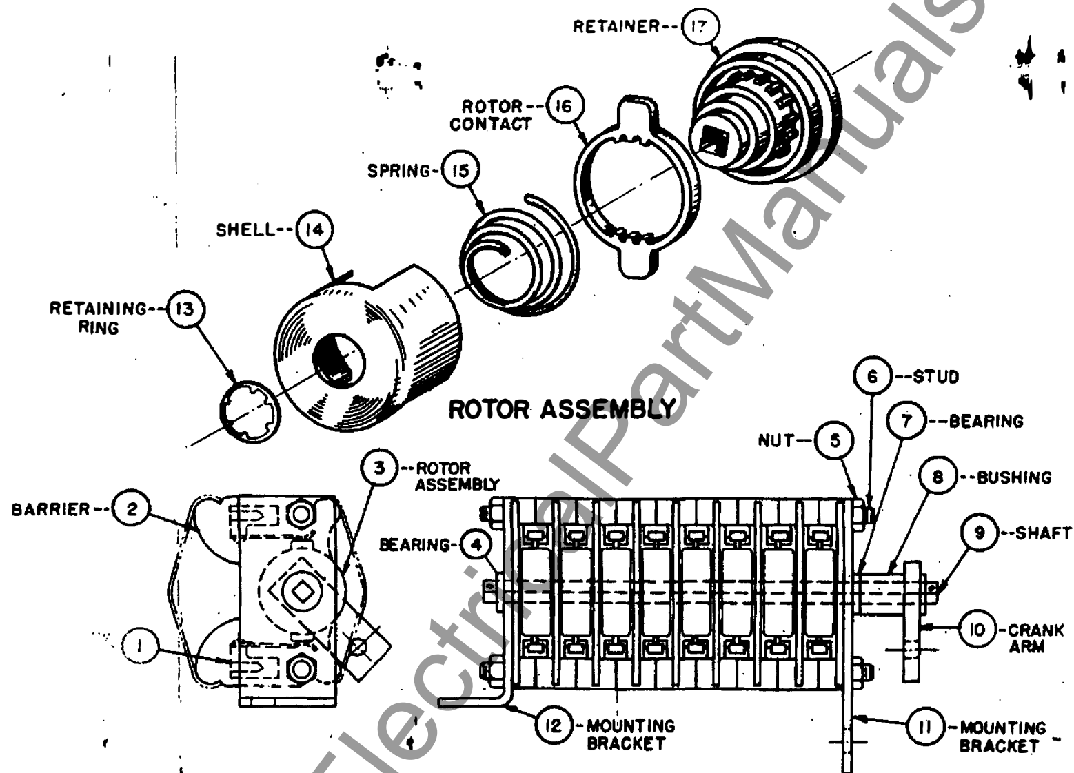
FIG. 11 TYPICAL AUXILIARY SWITCH
