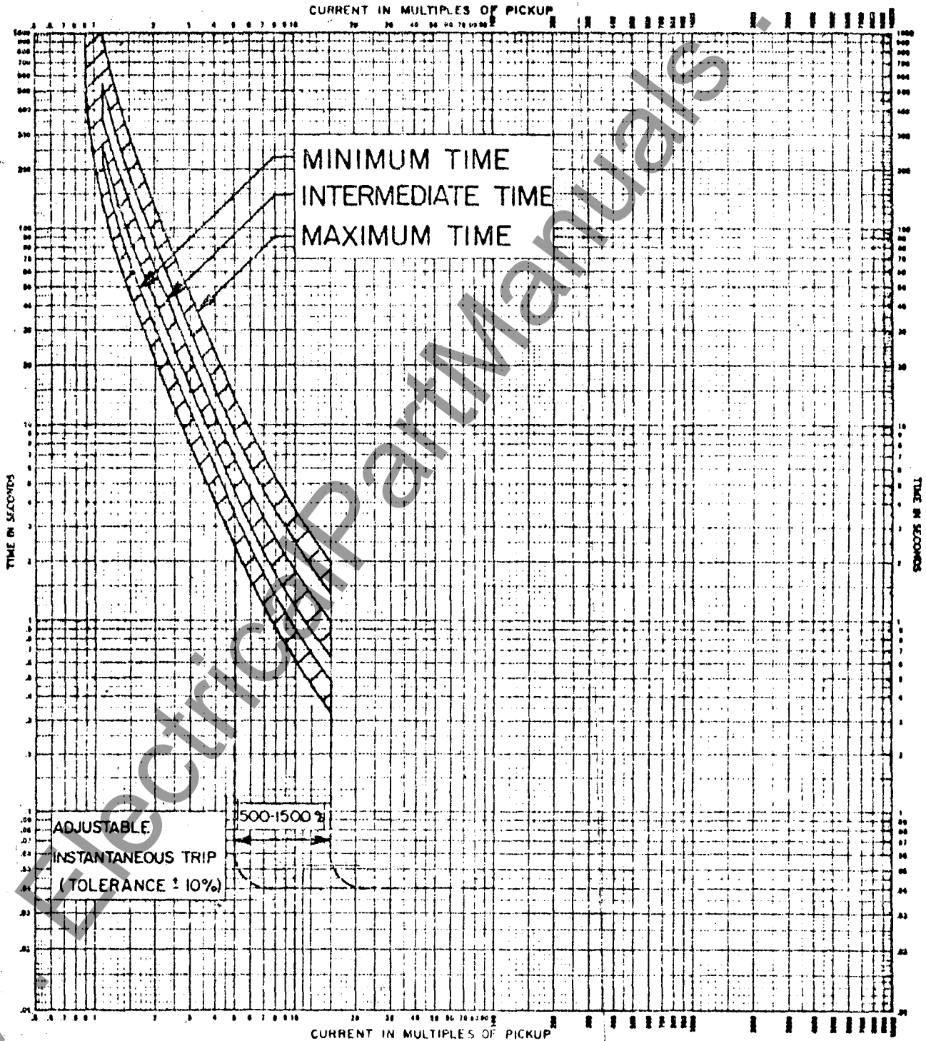
DUAL STATIC OVERCURRENT TRIP DEVICE - MODEL "A", "A-1", "A-G", "A-2", "AG" JANUARY 13, 1964 TYPICAL CURVE 71-240-558-404
