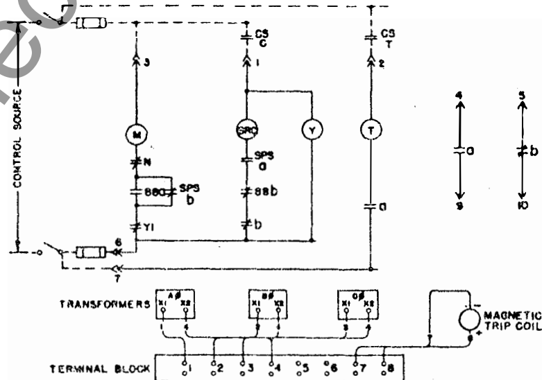
TYPICAL WIRING DIAGRAM FOR ELECTRICALLY OPERATED BREAKERS FIG.3
