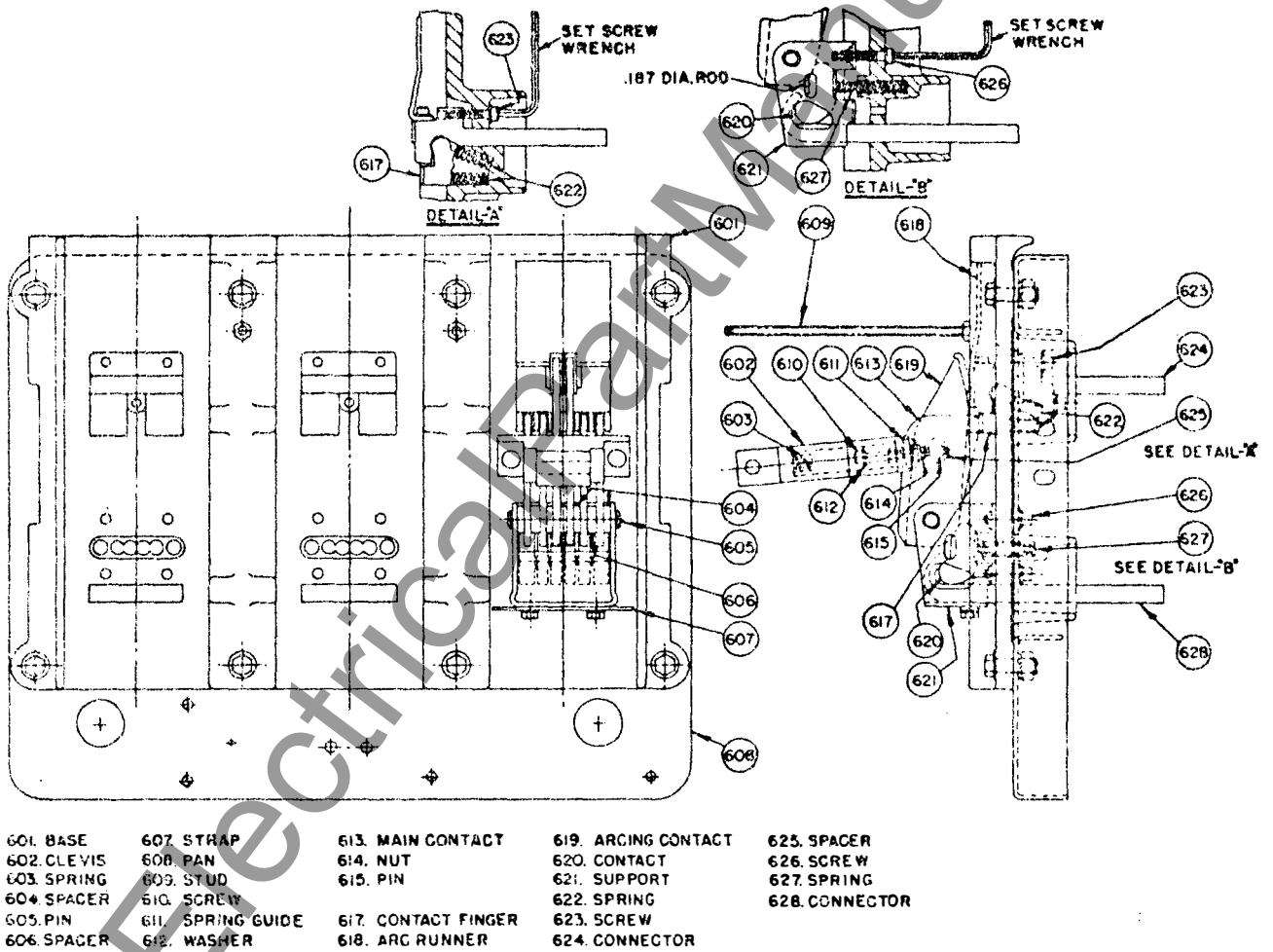
FIG. 6 TYPICAL PANEL ASSEMBLY MARCH 8, 1967 72-340-021-401
