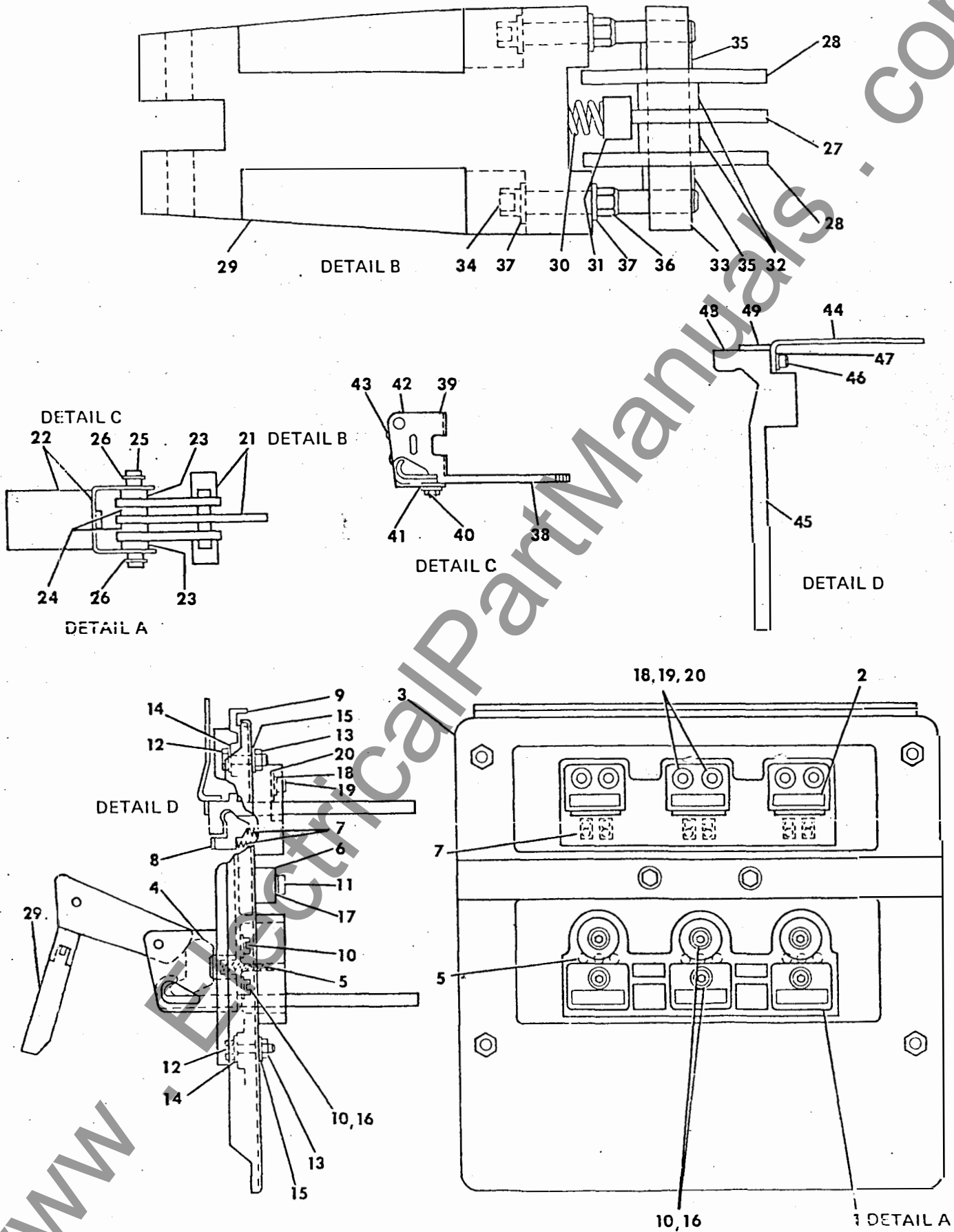
Figure 3. Panel Assembly (18-657-346-522)
