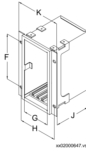
Figure 20: Case without rear cover with 19" rack mounting kit
