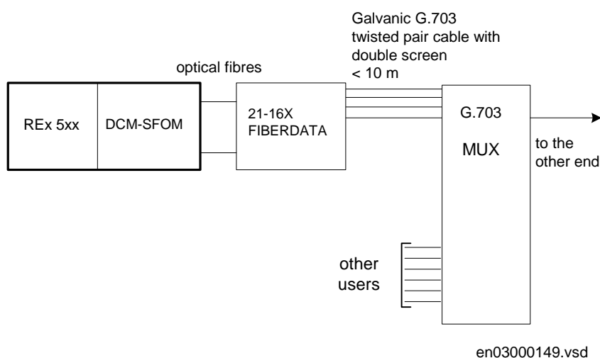
Figure 14: Multiplexed link, optical fibre - galvanic connection G.703 with 21-16X
