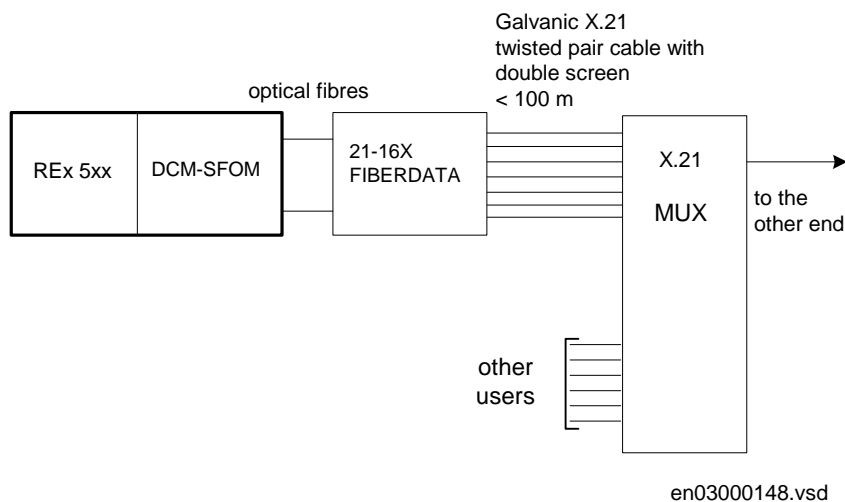
Figure 13: Multiplexed link, optical fibre - galvanic connection X.21 with 21-16X
