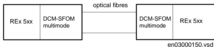
Figure 2: Dedicated link, short range optical fibre connection
