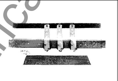
800-Amp contactor load or line stab assembly, complete with mounting
