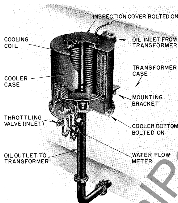
FIG. 1. Cutaway View of "OW" Cooler Individually Mounted on Transformer.
