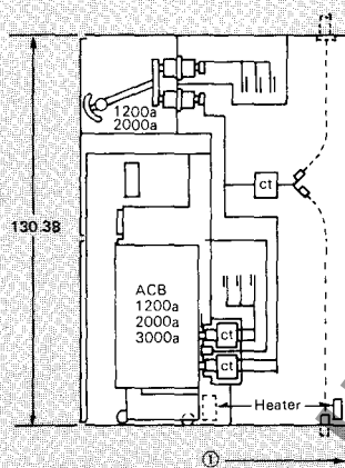
Transfer Bus with Disconnect Switch
