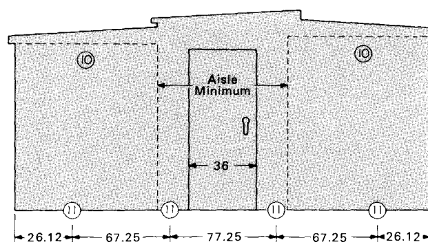
Common Aisle Shelter for-M
