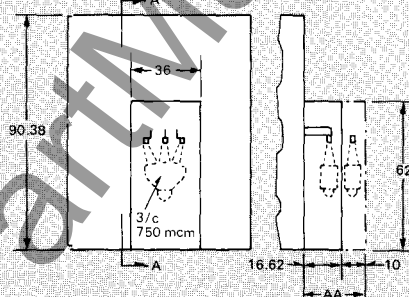
End Entrance Compartment
