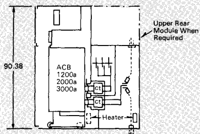
Feeder or Incoming Line
