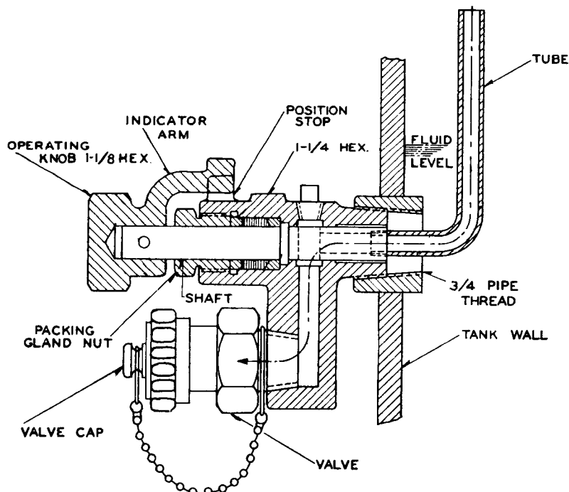
FIG. 2—WESTINGHOUSE ROTARY TYPE SAMPLING VALVE SECTIONAL VIEW
