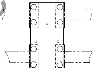
Fig. 6 Baseplate: Double crossarm or platform mounting (3-72 KV)
