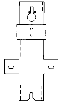
Fig. 4 Pole Mounting Bracket: Single arrester horizontal mounting (3-36 KV)
