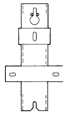
Fig. 4 Pole Mounting Bracket: Single arrester horizontal mounting (3-36 KV)
