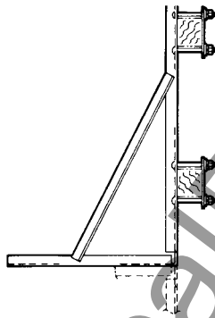
Fig. 2 Double crossarm bracket, reversible (3-72 KV).
