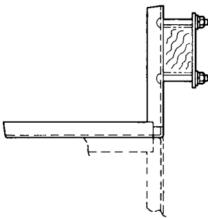
Fig. 1 Single crossarm bracket, reversible (3-39 KV)
