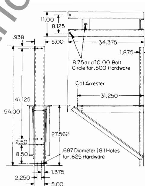
S#279C251A10 O.D. 6463A11 Wall Mounting Bracket
