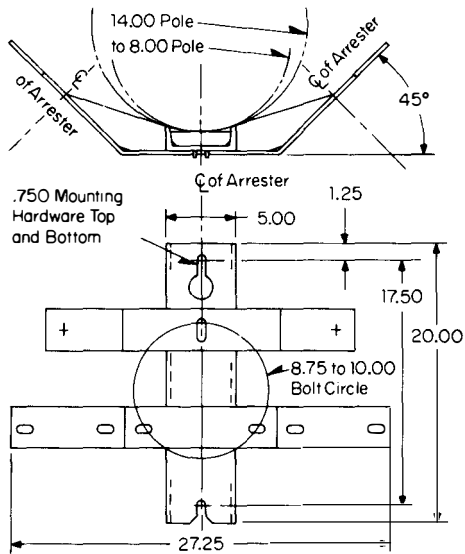
S#279C251A01 O.D. 5572A78 Pole Mounting Bracket: Three Arresters Horizontal Mounting
