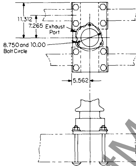
S#279C251A09 O.D. 6463A10 Baseplate: Double Crossarm or Platform Mounting
