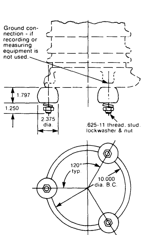
S#8044A96A01 Insulating Base (Post Type) for 3 - 48 KV SMX Arresters
