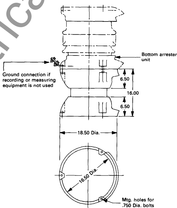
S#898A945A01 Insulating Unit for SMX Arrester 588-612 KV
