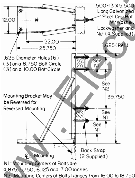
S#279C251A07 O.D. 6463A08 Double Crossarm, Reversible Mounting Bracket
