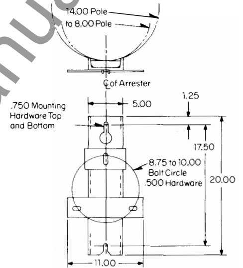
S#279C251A02 O.D. 5572A79 Pole Mounting Bracket: Single Arrester Horizontal Mounting
