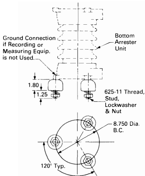
S#8046A07A01 O.D. 9242A85 Insulating Posts For IMX Arrester (3-120 KV)
