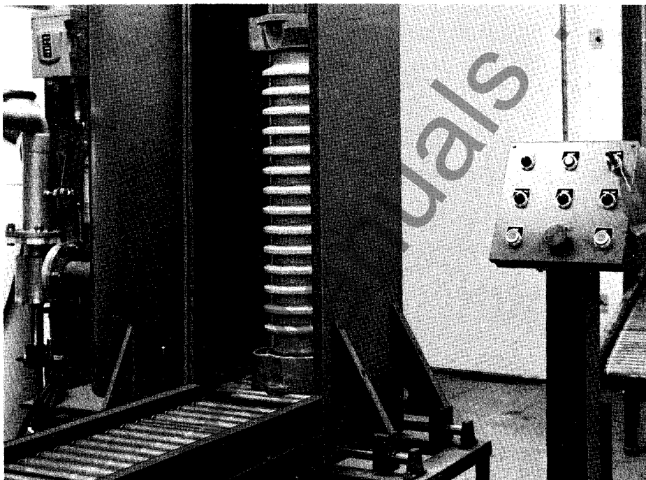
Seal Testing of a IVL Arrester
