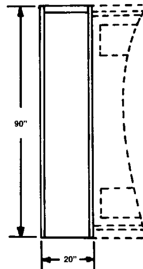
Front Elevation
