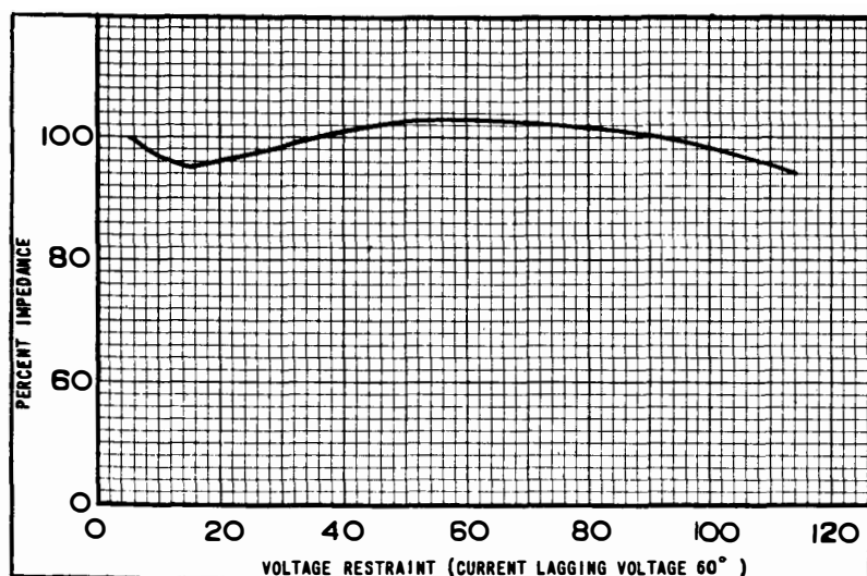
Fig. 4. Typical Impedance Curve of the Impedance Unit. (HZ)
