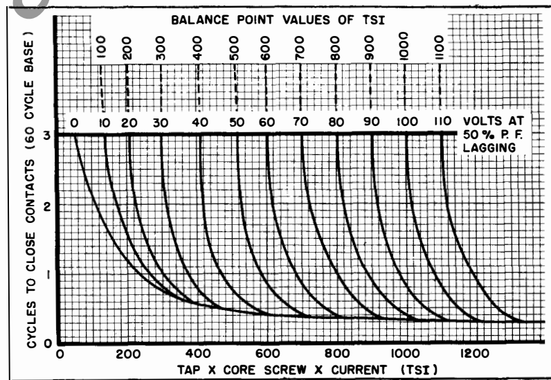
Fig. 7. Typical Time Curves of the Impedance Unit (HZ)
