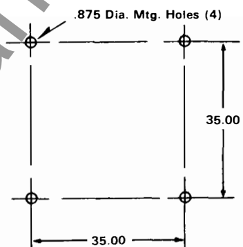
Mounting Base Plan
