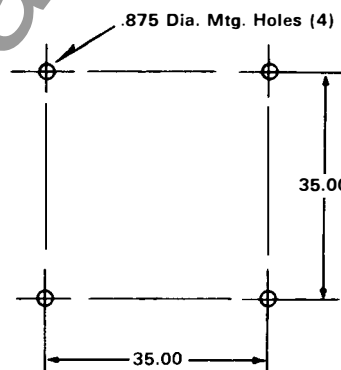
Mounting Base Plan
