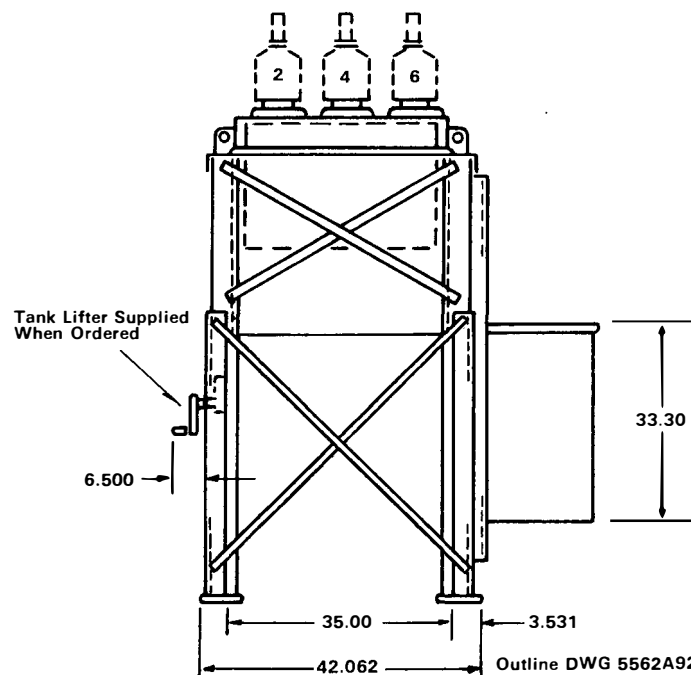
Outline DWG 5562A92
