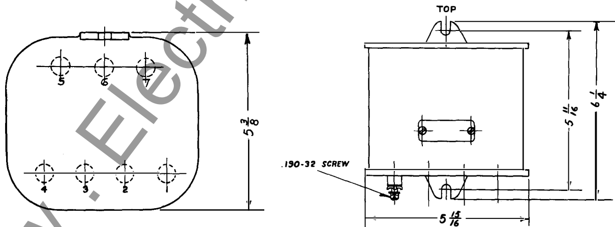
Fig. 3. Outline and Drilling Plan of the Type CBU Current Blocking Unit Case. (For reference only)
