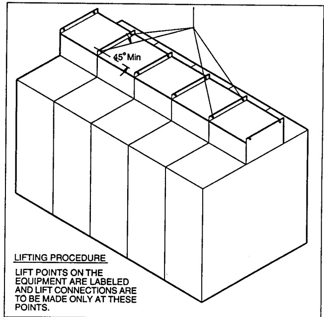
Figure 2. Lifting Indoor Switchgear
