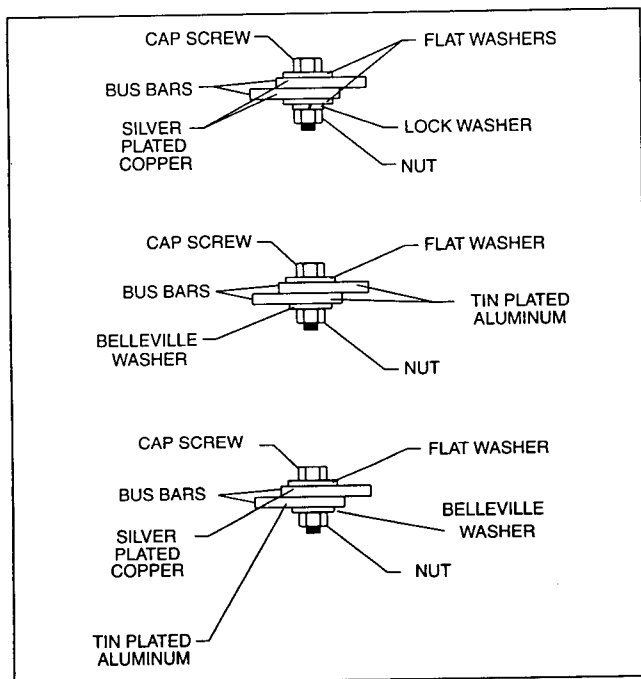
Figure 15. Bus Joint Hardware Installation
