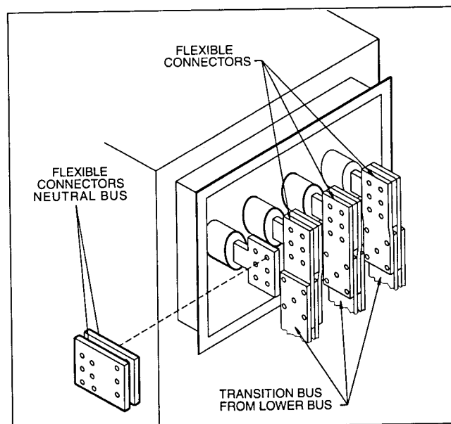
Figure 16. Transformer Throat Connection (Lower Bus Shown, Upper Bus Similar)
