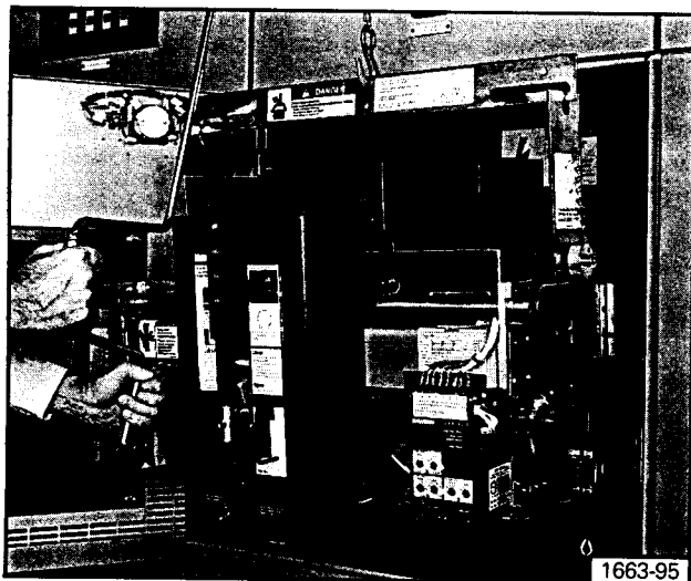
B) Attach crane hook and insert crank into hoist mechanism eye. Raise breaker above compartment, and fully extend rails.
