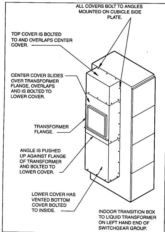
Figure 17. Transformer Hood
