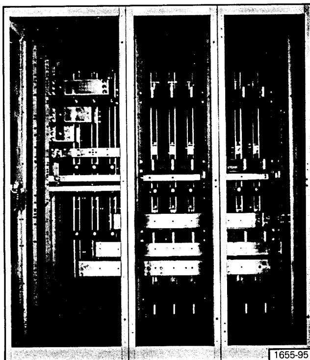
Figure 13. Typical Bus Bar Arrangement
