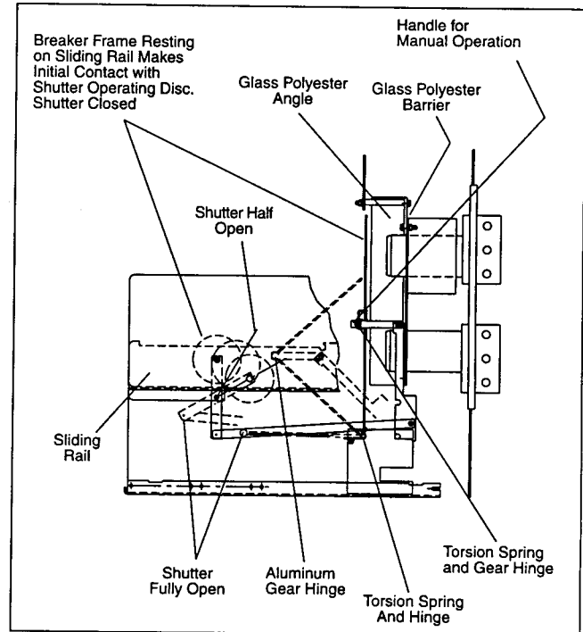
Figure 24. Metal Shutter
