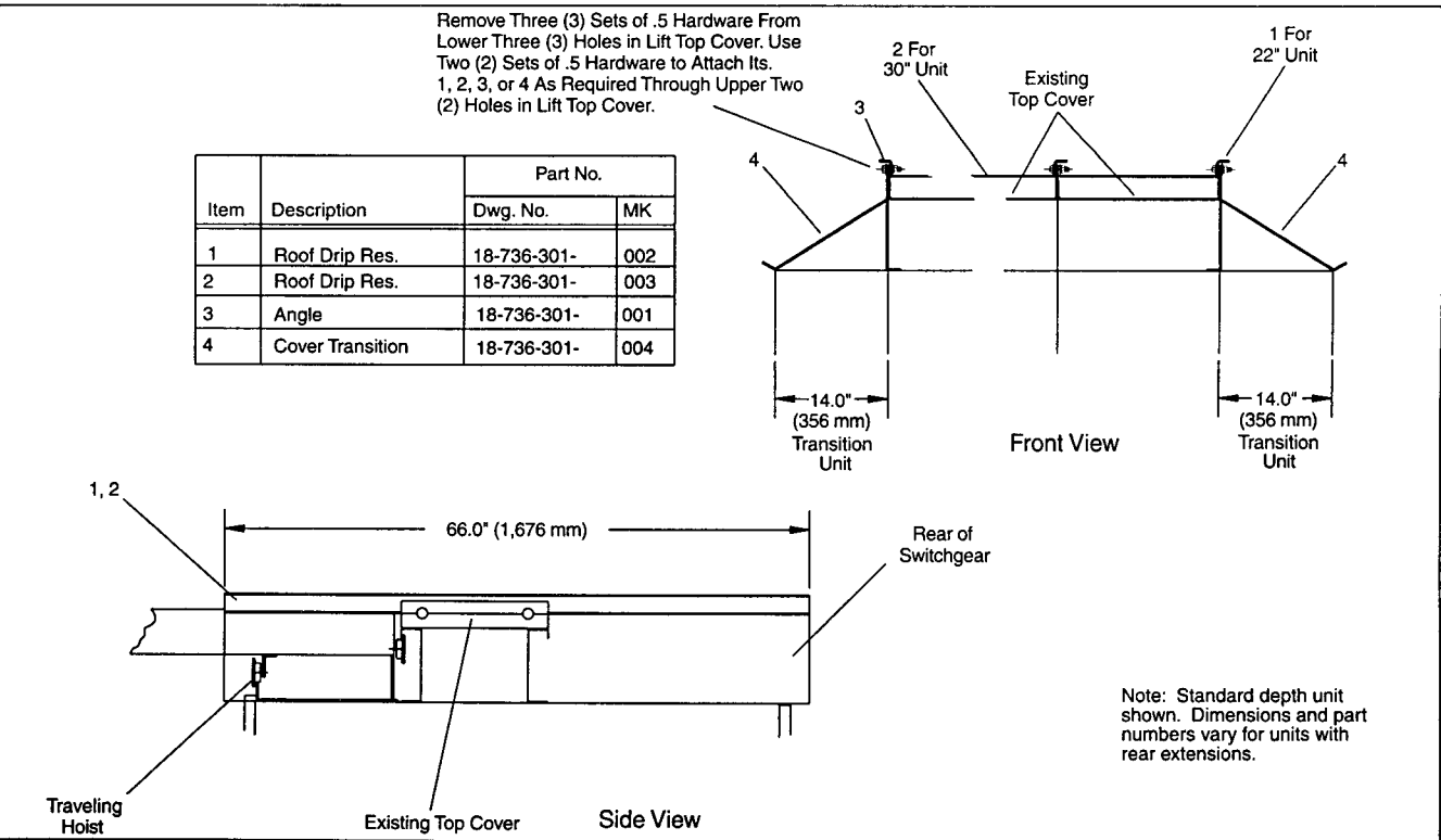
Figure 29. Drip Resistant Shield Option
