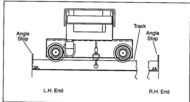
Figure 12. Traveling Crane
