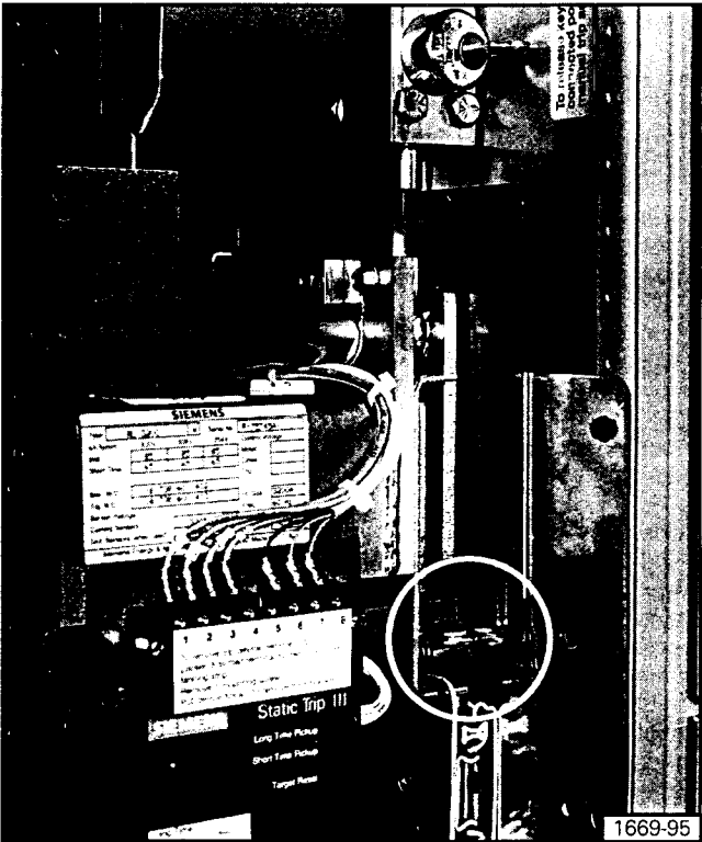
Figure 28. Key Interlock Option (Circle shows that interlock has blocked closing of circuit breaker)
