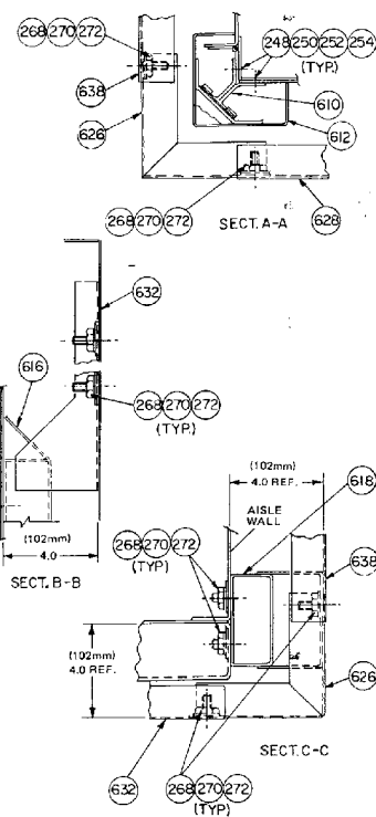
Figure 15. Trim Arrangement - Type "SIV" Single Aisle
