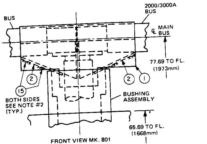
TYPICAL 2000/3000A INTERMEDIATE UNIT BUS INSULATION COVERS. (GOOD FOR A, B OR Cφ)
