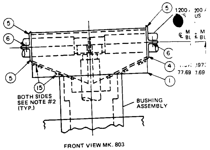
TYPICAL 1200A INTERMEDIATE UNIT BUS INSULATION COVERS. (GOOD FOR A, B OR Cφ)
