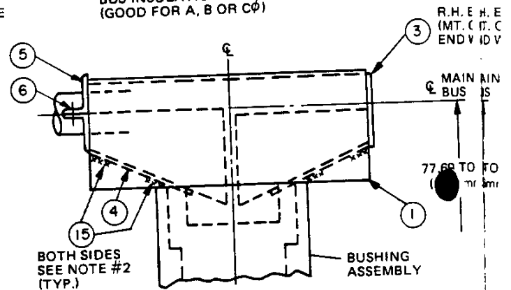
TYPICAL 1200A END UNIT BUS INSULATION COVERS L.H. END OR R.H. END (GOOD FOR A, B OR Cφ)
