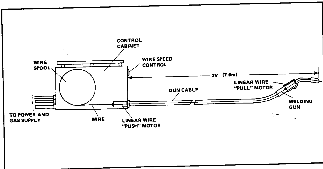
Figure 21. Schematic of Typical Wire Feeding System
