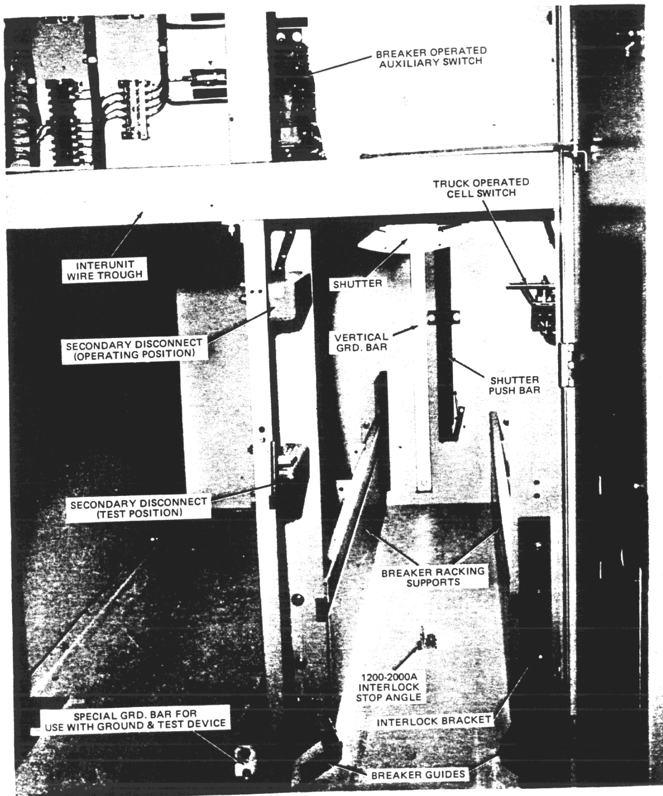
Figure 36. Positioning Interlocking and Operating Devices
