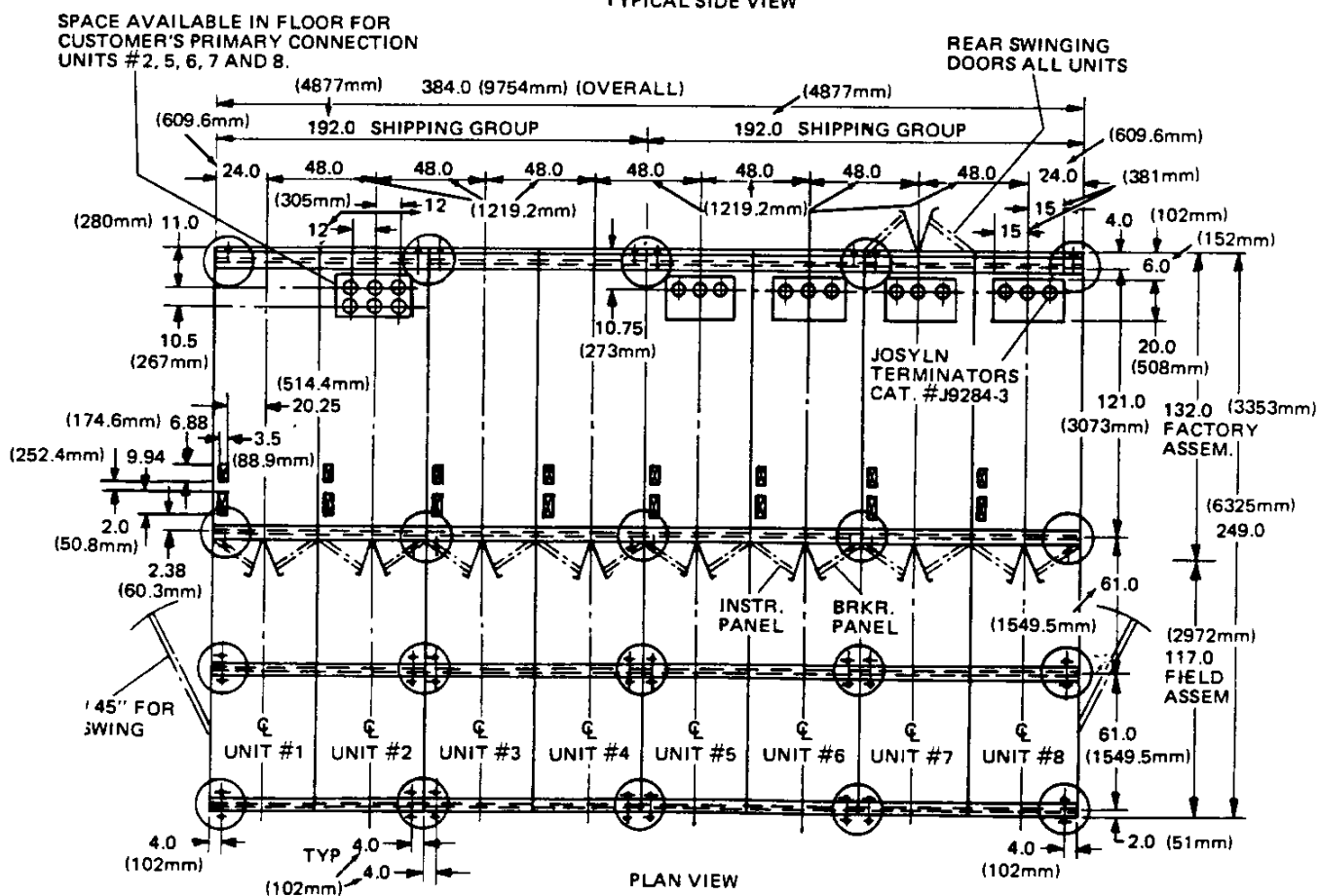
Figure 10. Floor Plan and Typical Side View of 34.5 kV Single Aisle Shelter-Clad Cubicle
