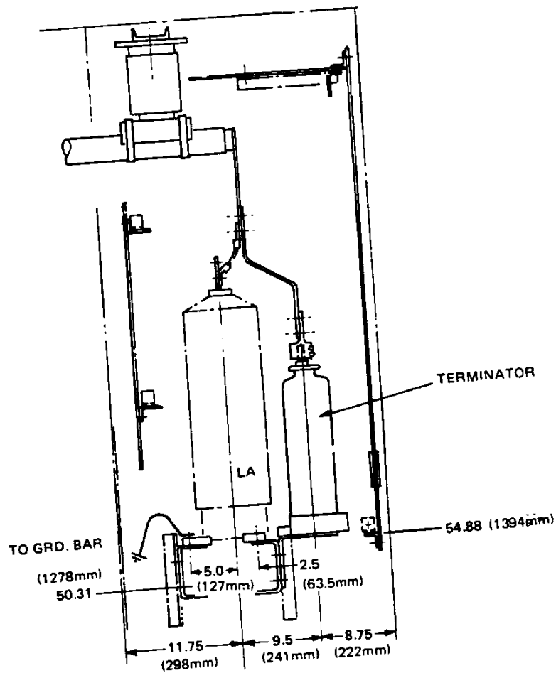
Figure 27. Porcelain Top Lightning Arrester and Terminator Mounting
