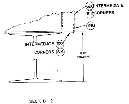
Figure 19. Trim Arrangement — Type "SIV" Common Aisle
