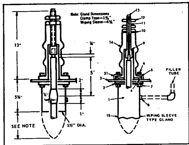
Fig. 14 - Single-conductor potheads.
