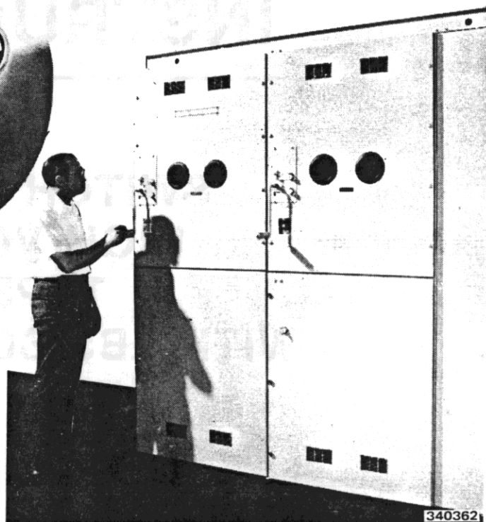
Fig. 2 - Indoor switch cubicle group arrangement.
