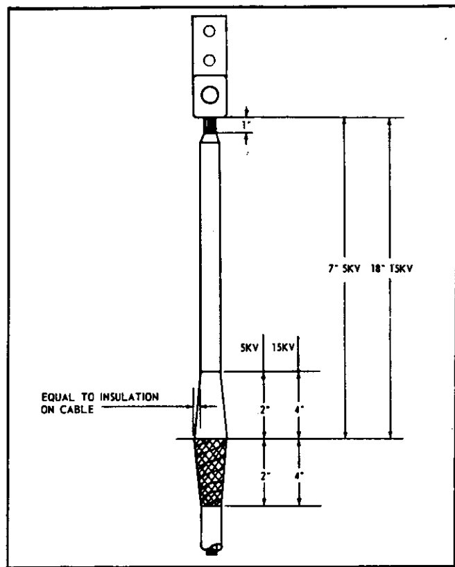
Fig. 9 - Typical customer's cable connections.
