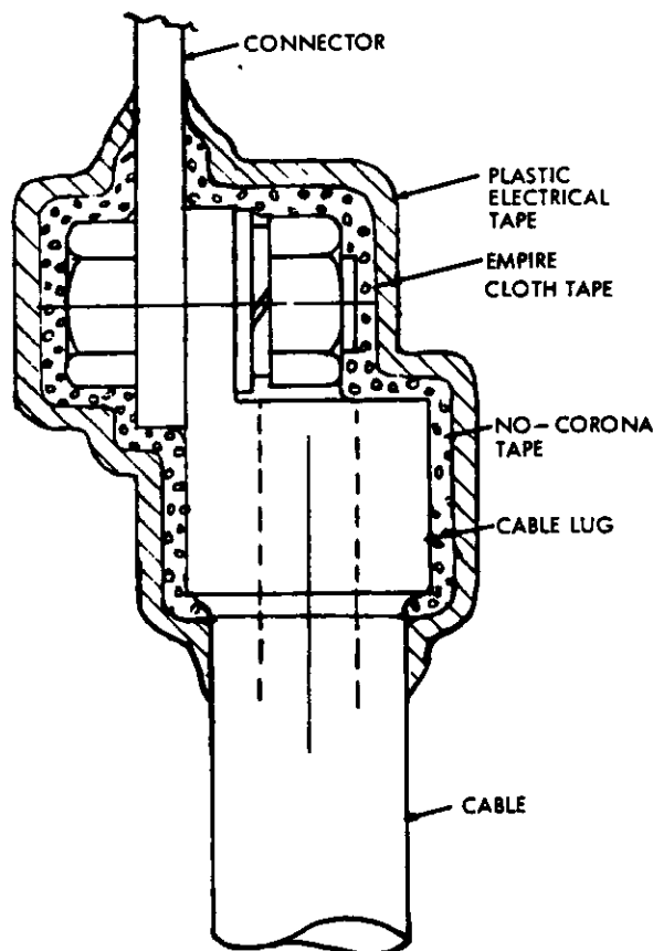
Fig. 17 — Example of joint taping for cable connections required only on 15-kv selector switch.
