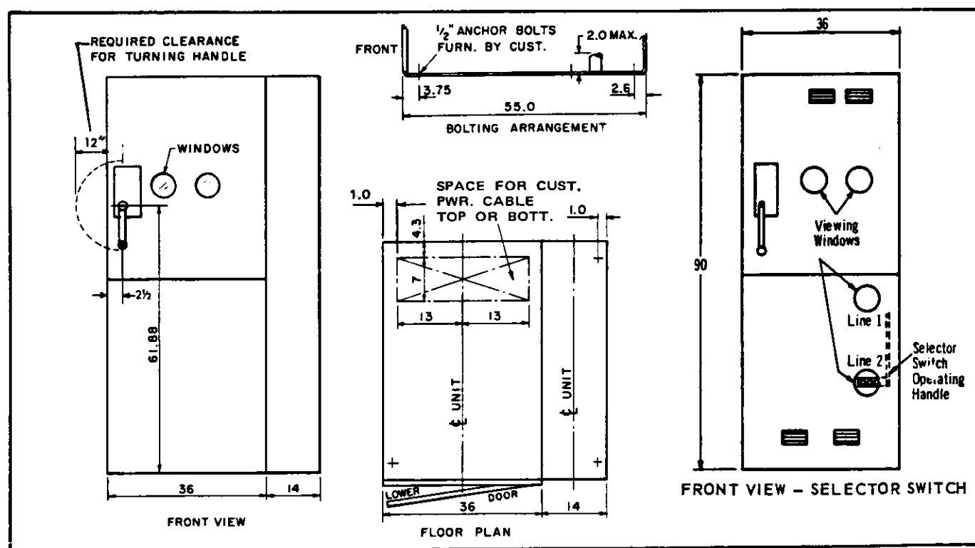
Fig. 3 - Indoor floor plan arrangement and bolting.
