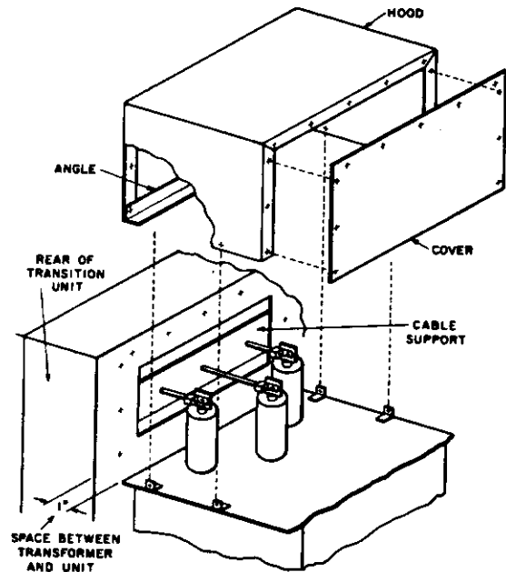
Fig. 5 — Flexible cable connections to the transformer, protected by a hood assembly (above).
