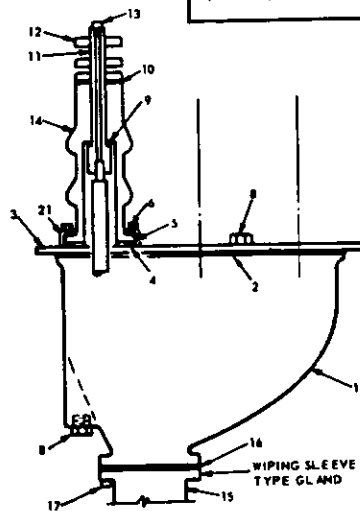
Fig. 13 - Three-conductor potheads.
