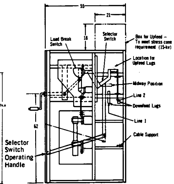
Fig. 8 - Upfeed or downfeed connection-selector switch.
