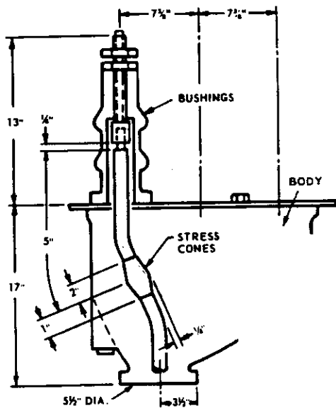
Fig. 13 - Three-conductor potheads.
