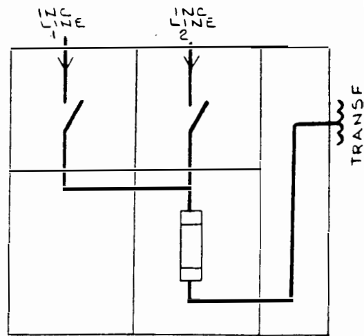
FIG. 5 DOUBLE UNIT LVPS
