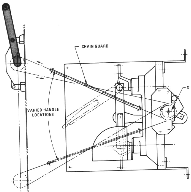
Fig. 11 Handle "UP" in switch closed position.
