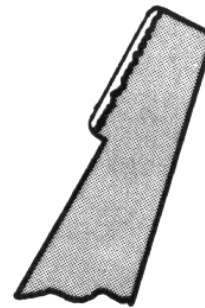
Fig. 27 End of auxiliary quick-break blade showing erosion at arcing tip
