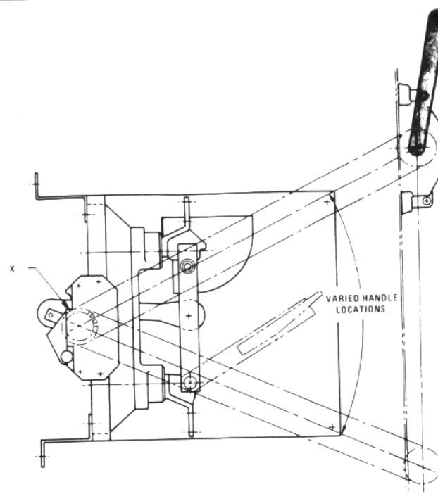
Fig. 1 Handle "UP" in switch closed position.
