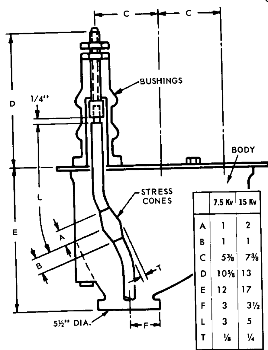
Fig. 11 — Three-conductor potheads.
