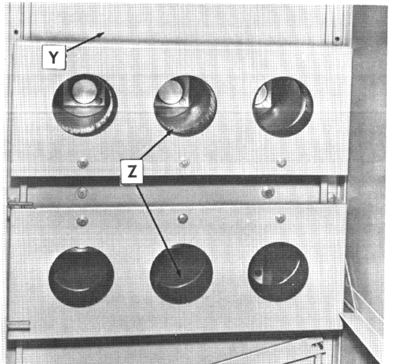
Current transformers (Z) shown mounted on both bus and load side. Shutter (Y) blocked open to show disconnect studs.
