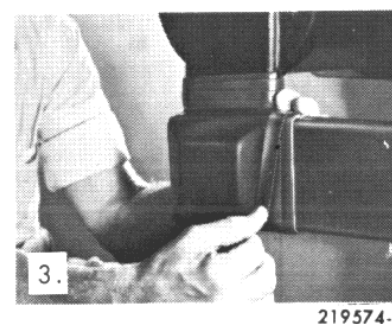
Fig. 7 — Molded polyvinyl boots are used to insulate bus joints of 13.8-kv switchgear. Molded boot is placed over bus joint (1, 2) and then (3) secured over bolted bus joint with vinyl tape.
