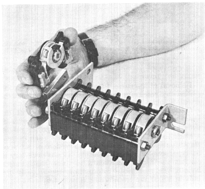
Fig. 28 — Only a pair of pliers is necessary to adjust each Q-10 auxiliary switch stage. Each point of a stage can be individually adjusted in 15 degree steps.
