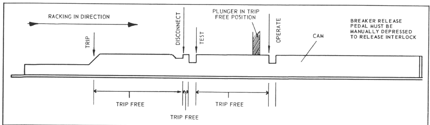
Fig. 16 — Guide track and interlock mechanism.
