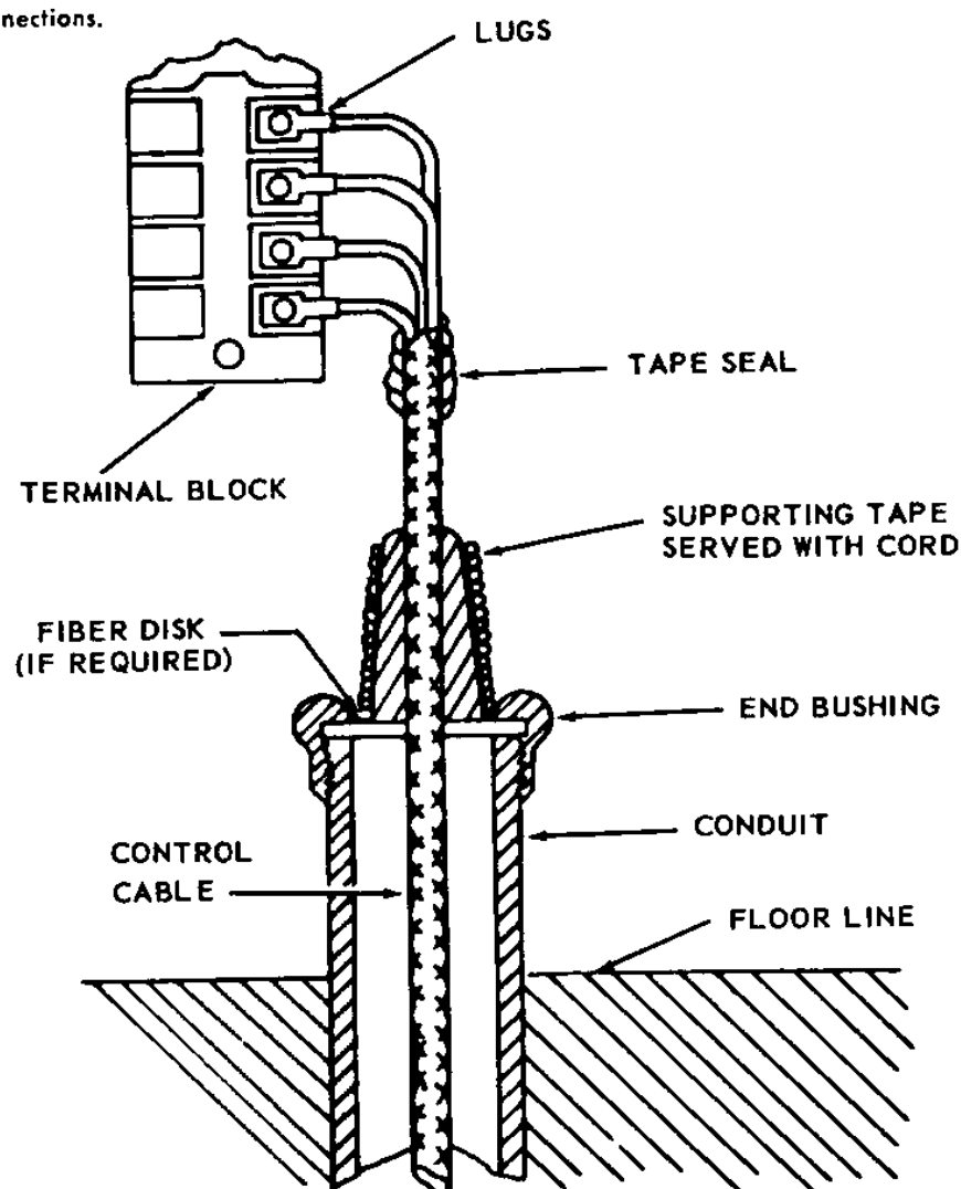
Fig. 15 — Secondary control cable connections.
