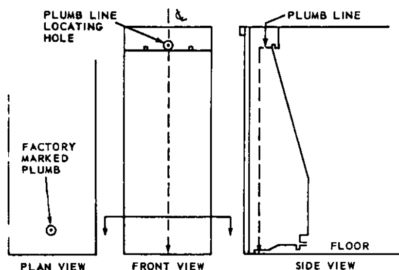
Fig. 3 — Correct method of plumbing units.
