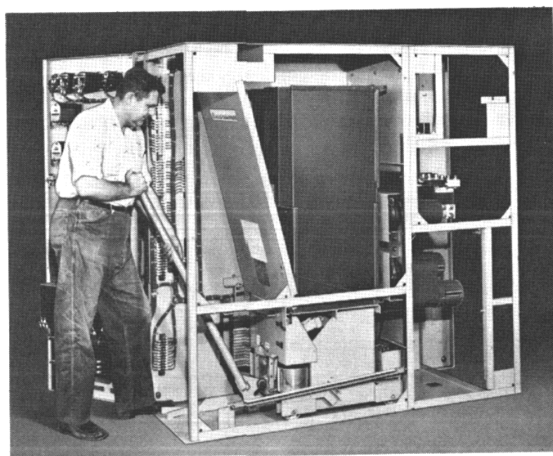
Fig. 19 — Racking instructions for 5-kv breaker. Top picture shows method of placing breaker in fully connected position and lower picture shows method used to rack breaker out of connected position.
