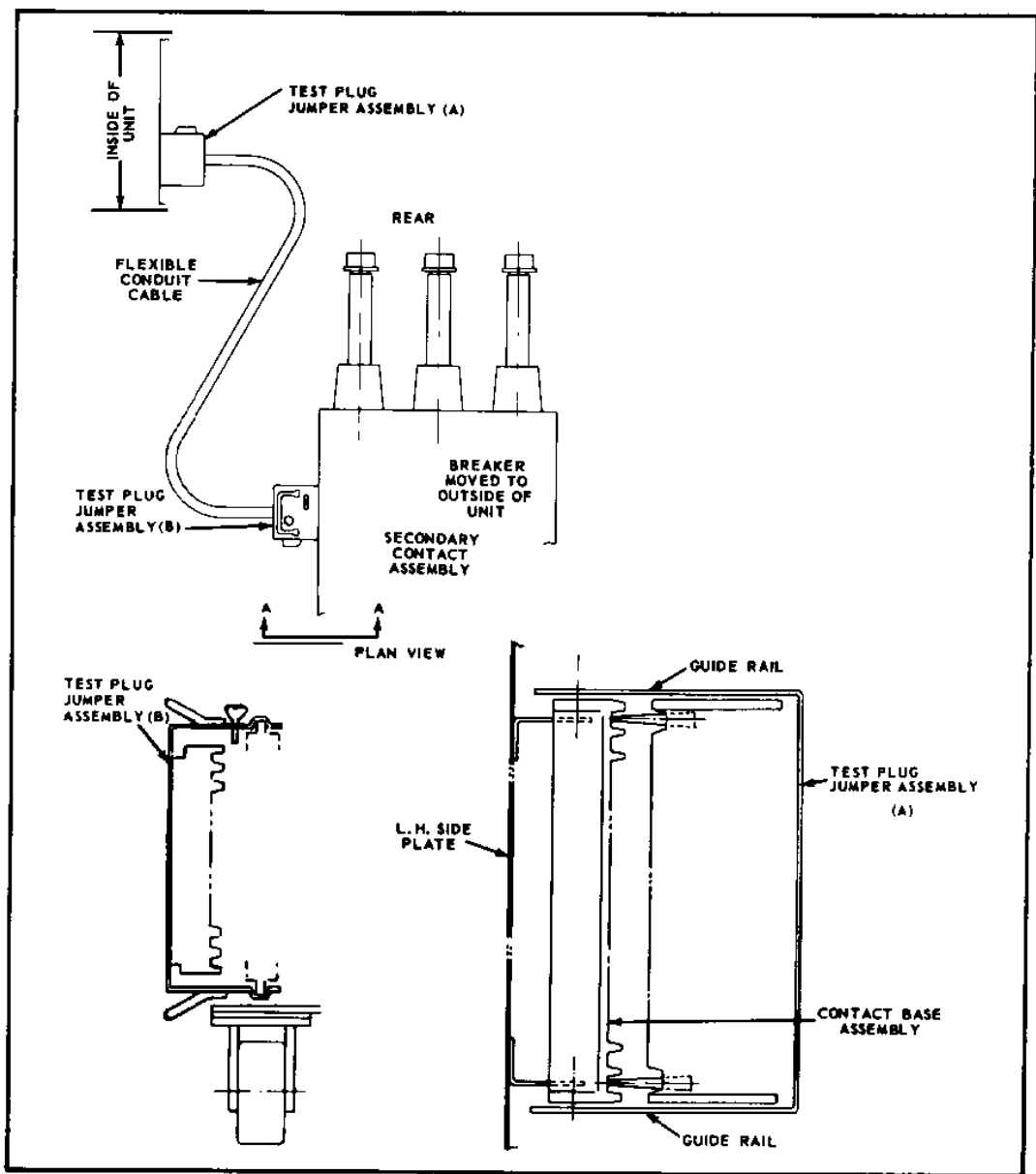
Fig. 31A — Plug jumper.
