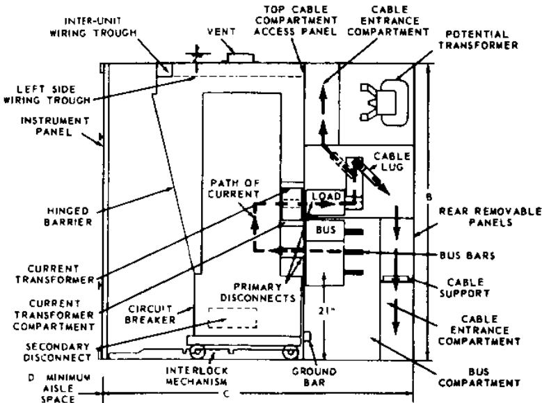
Fig. A — 5-kv Breaker Unit.
