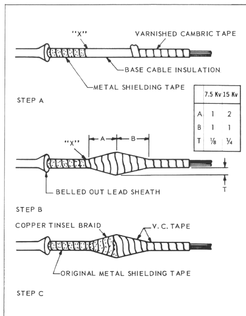
Fig. 9 — Typical cable and taped pothead connections.
