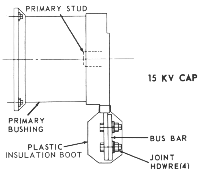
Fig. 6 — Bus joint using Pyro-Shield insulation caps (side views).
