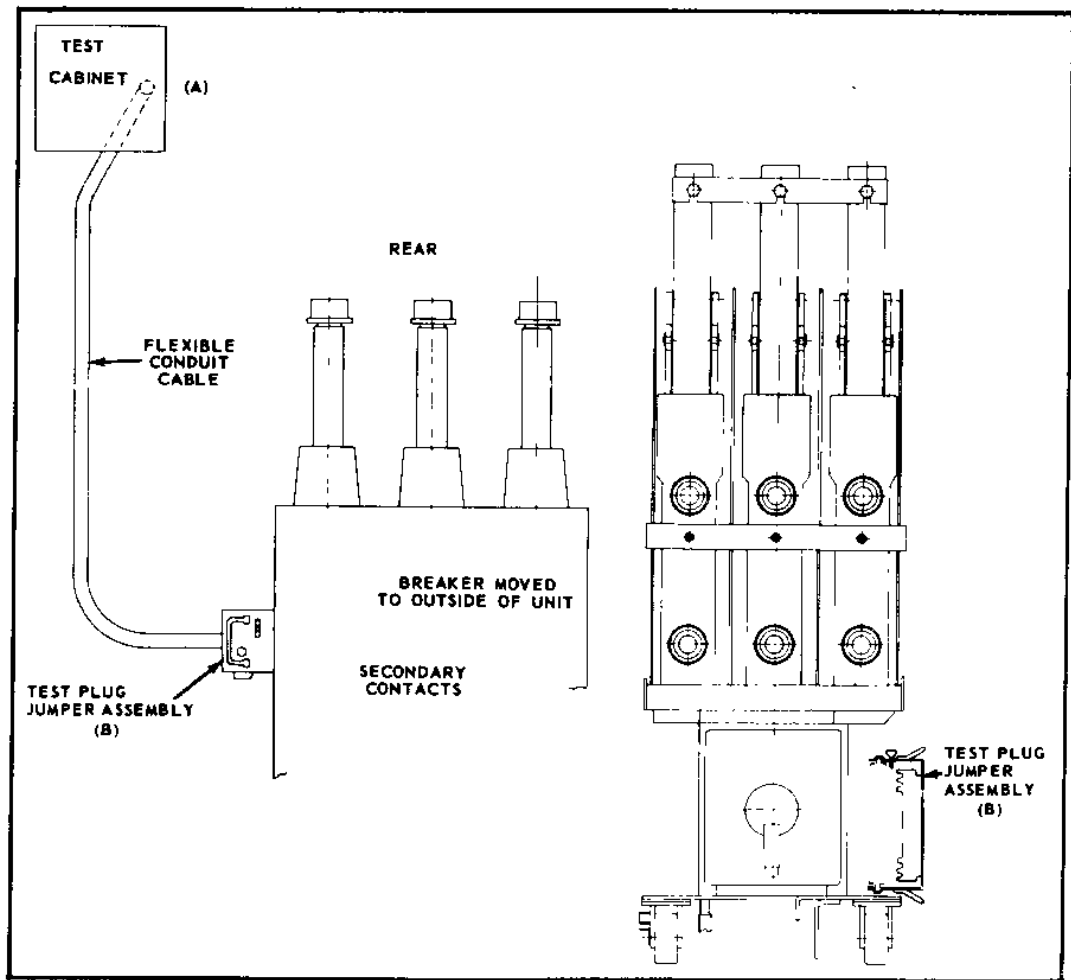
Fig. 31B — Optional test control cabinet.
