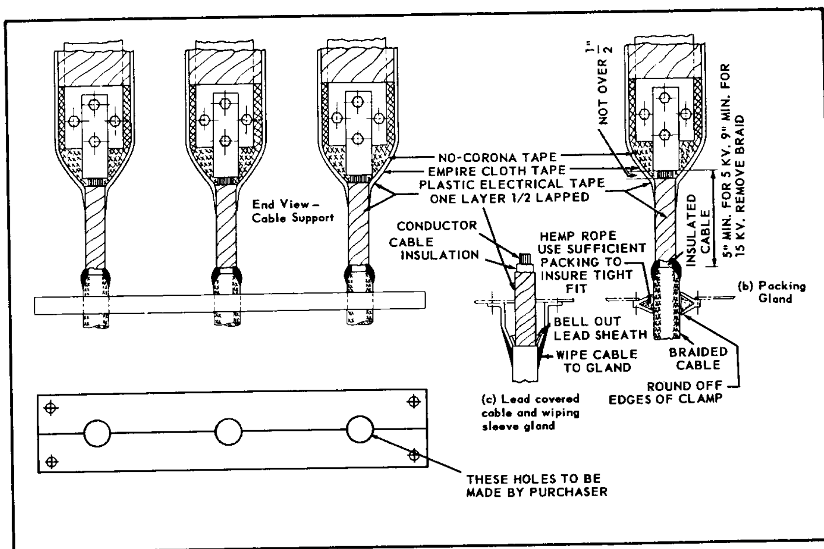
Fig. 14 — Primary cable connections.
