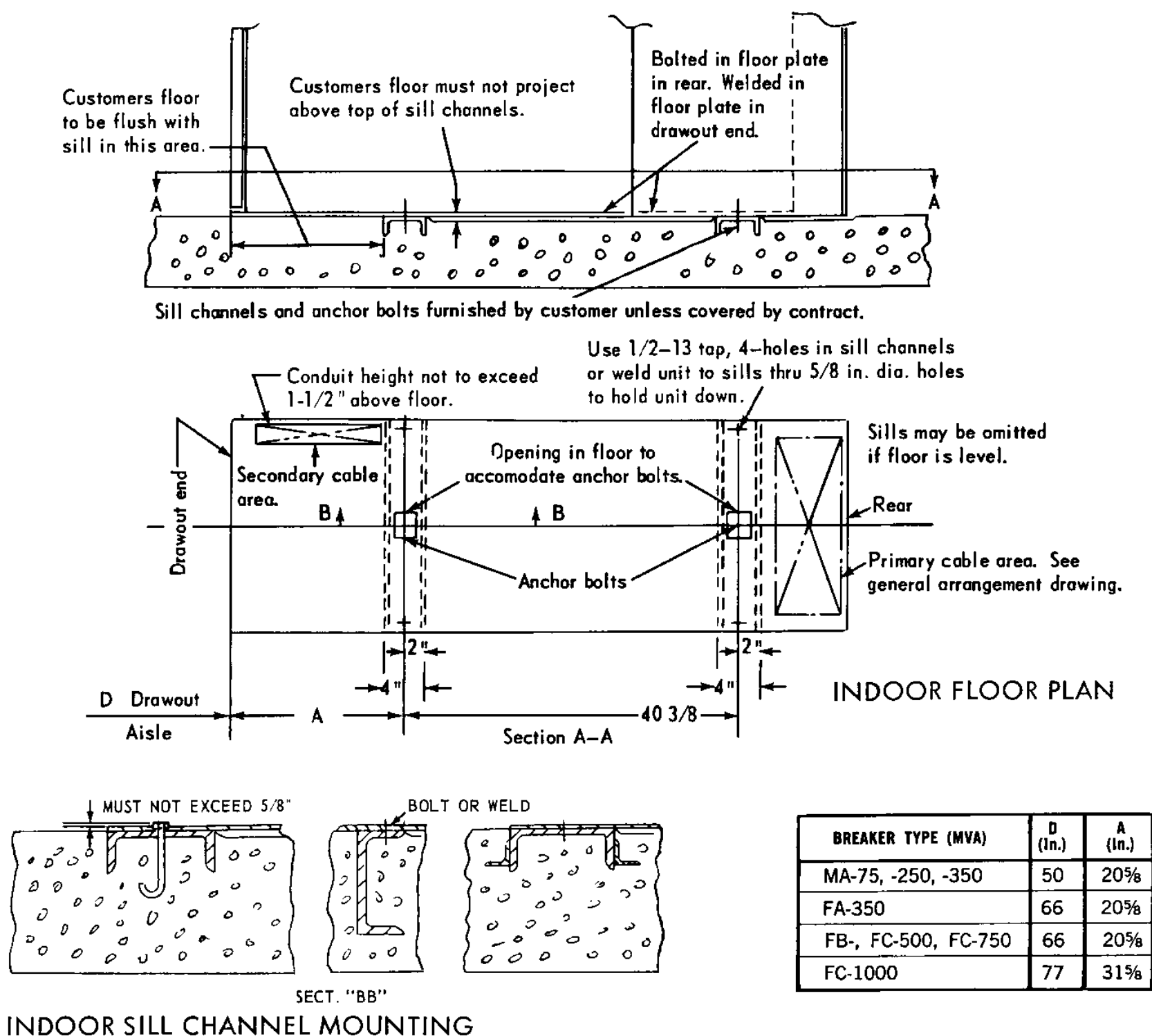
Fig. 2 — Typical floor plan and sill channel mounting.
