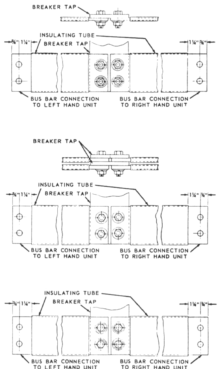
(5 OR 15 KV BUS) THRU BUS - VIEWED FROM OPPOSITE DRAWOUT
