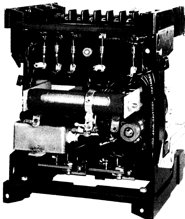
* Fig. 2. Type TT-12 Relay without case (Rear View)
