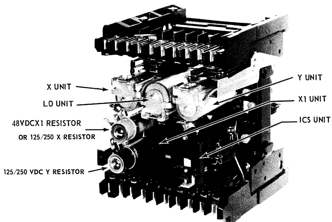
* Fig. 1. Type TT-12 Relay without case (Front View)
