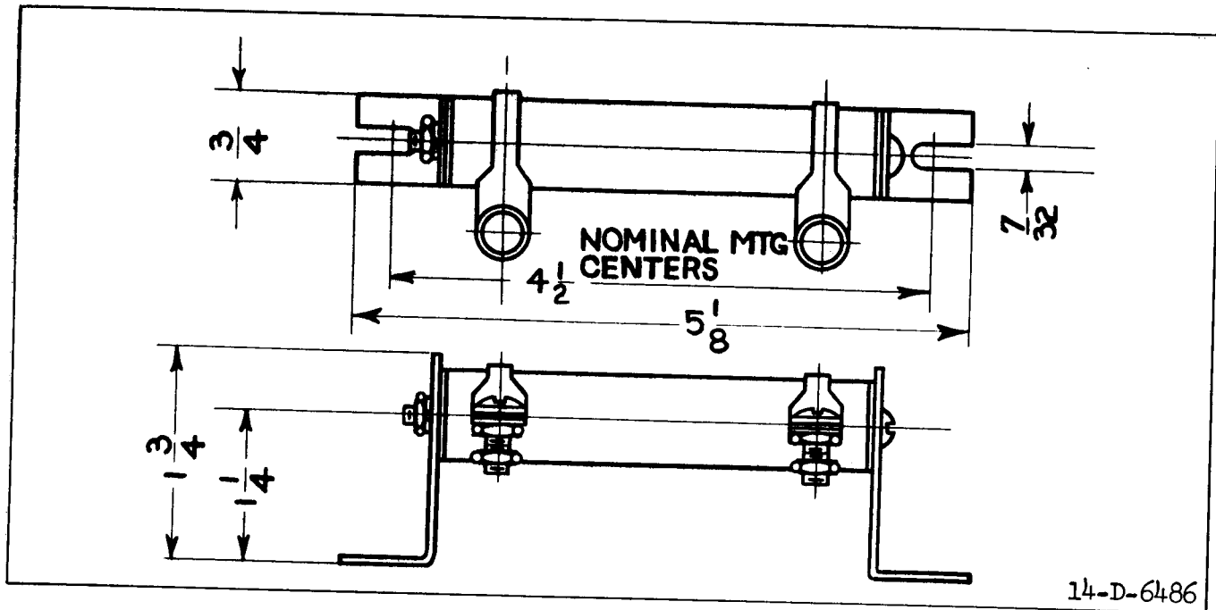
Fig. 4. Outline of the External Resistor.
