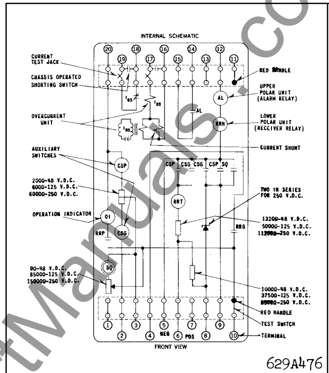
Fig. 3 Internal Schematic of the Type KA-4 Relay for TC carrier set.
