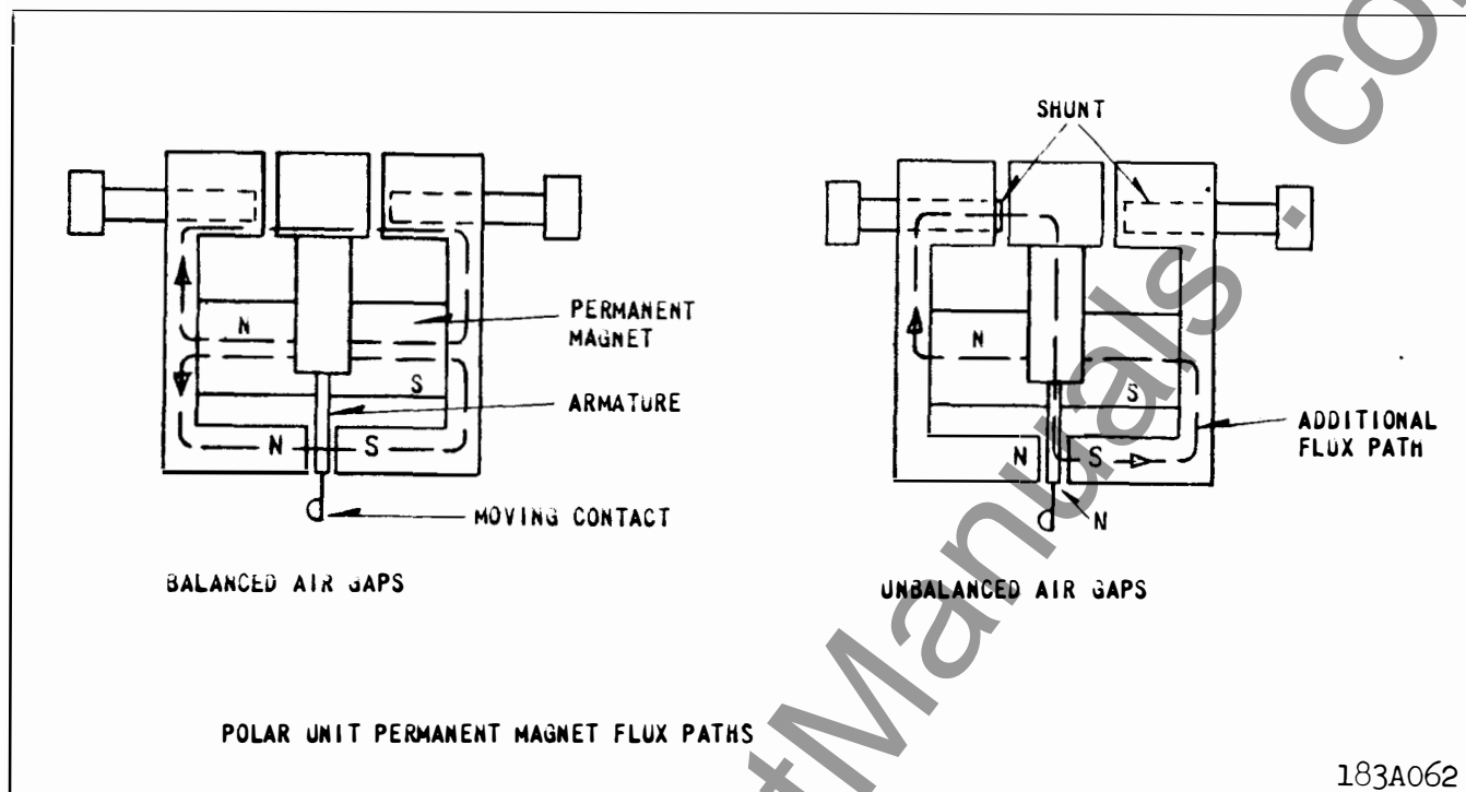
Fig. 5 Polar Unit Permanent Magnet Flux Paths.
