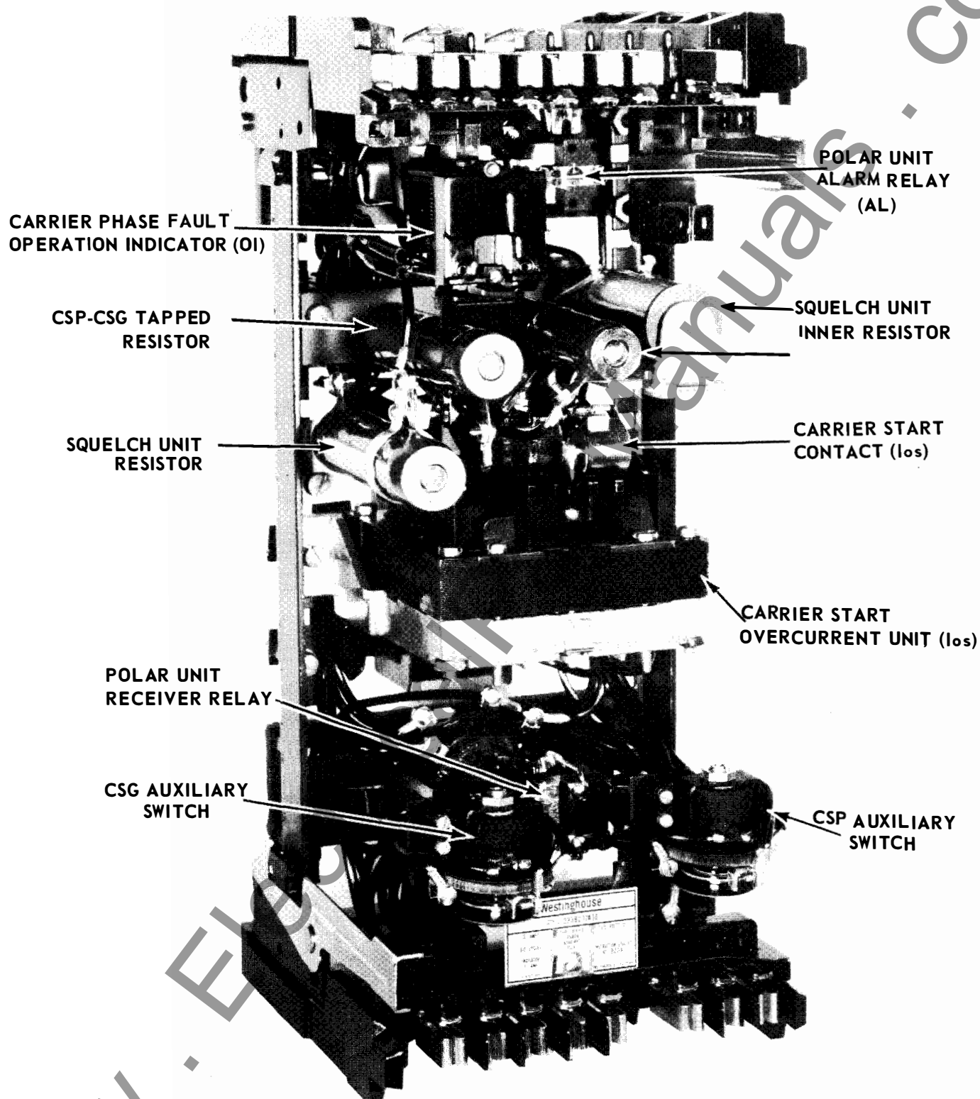
* Fig. 1 Type KA-4 Relay Without Case. (Front View)
