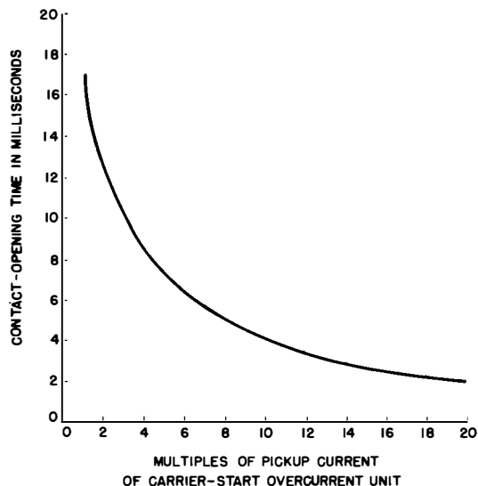
Fig. 4 Typical Time Characteristics of carrier start over-current unit of the type KA-4 Relay.
