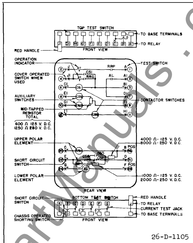
Fig. 1—Internal Schematic of the Type RS Relay in the Type FT Case for use in the Type HZ and HZM Carrier Scheme. Omit Test Switches for the Relay in the Standard Case.
