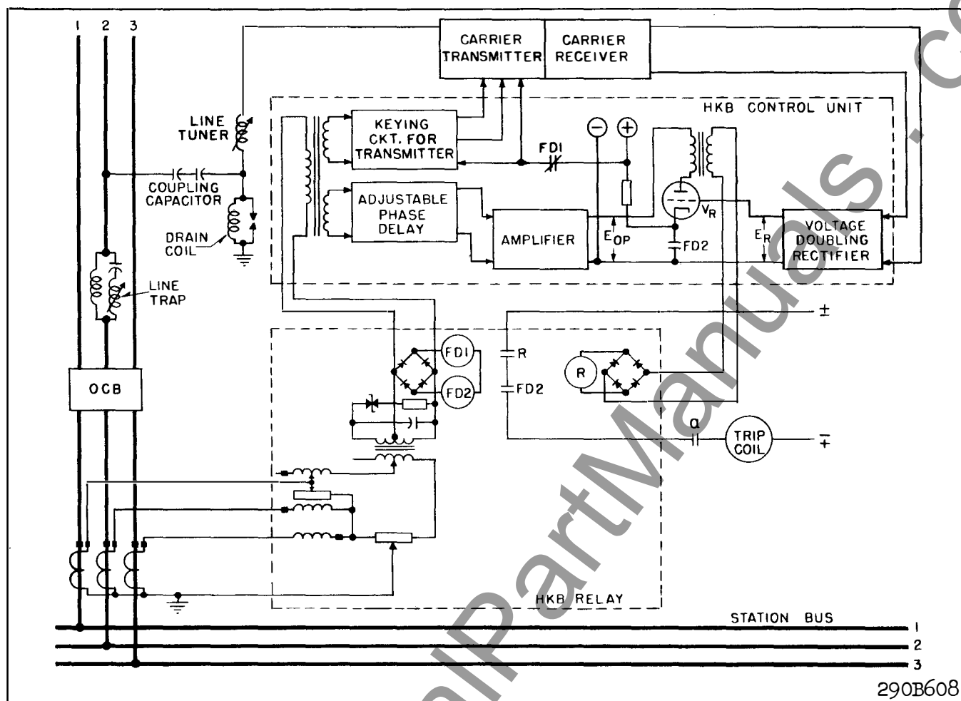
Fig. 1 - Basic Schematic Connections of the Type HKB Relaying System.
