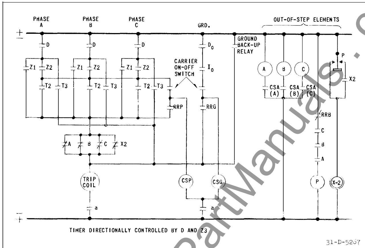
* Fig. 2—Simplified D-C Schematic of the Trip Circuits.
