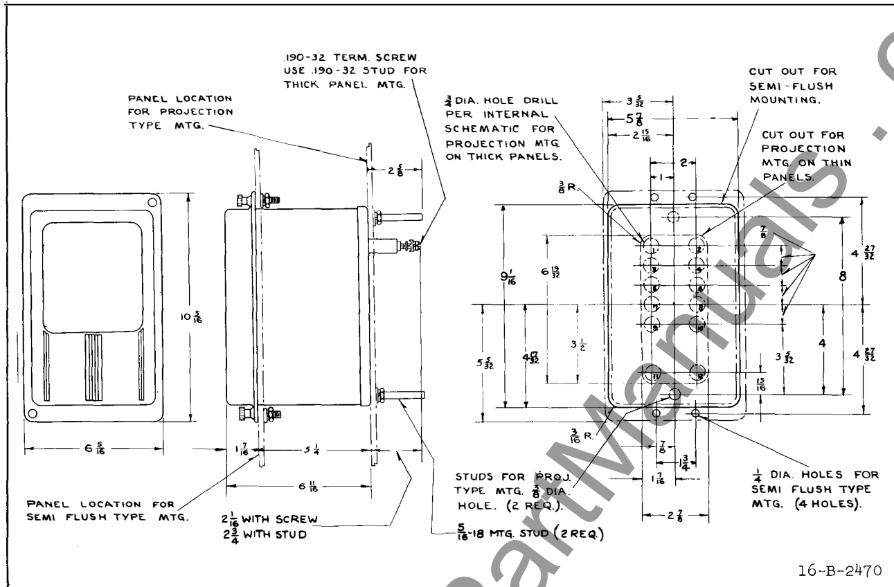
Fig. 8—Outline and Drilling Plan for the S10 Projection or Semi-flush Type FT Flexitest Case. (For Reference Only). See the Internal Schematic for the Terminals Supplied.
