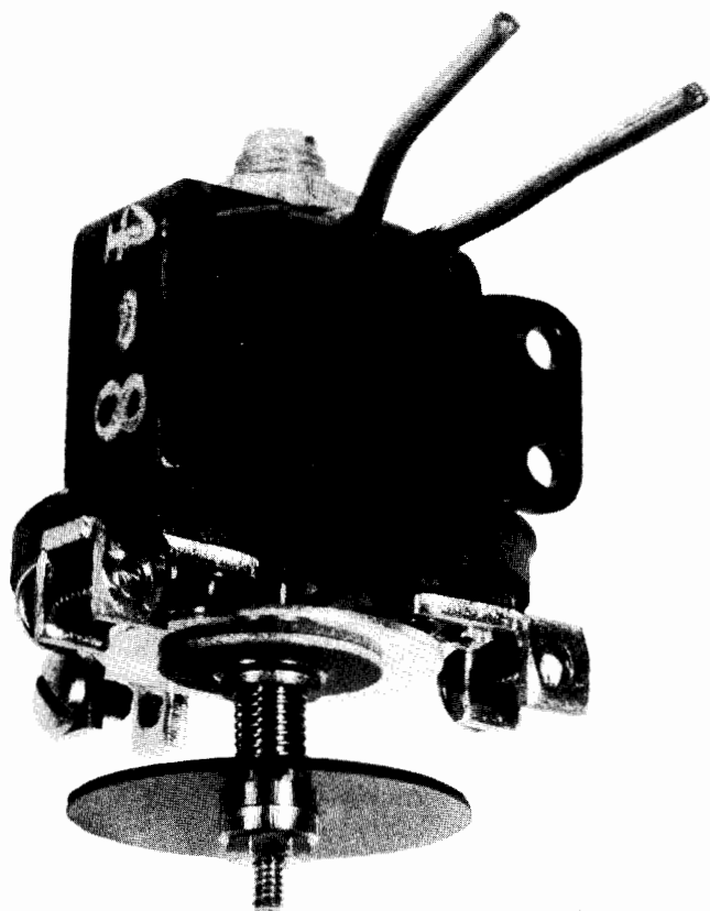
Fig. 1. High Drop-Out Instantaneous Trip Unit (ITH).
