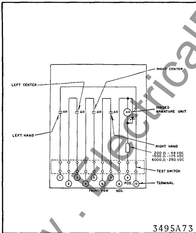
Fig. 5. Internal schematic of the Type AR Relay - High Threshold - with 4 make contacts in FT-11 case.
