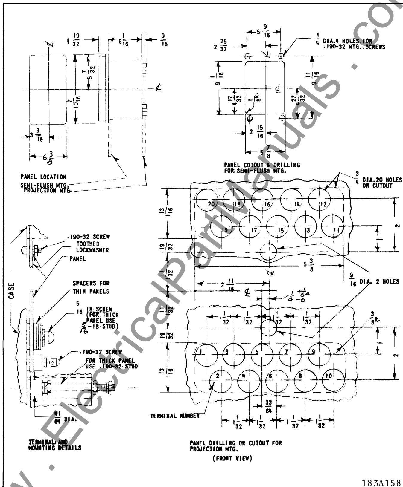
Fig. 13. Outline and drilling plan for the Type AR Relay in the FT-22 case.
