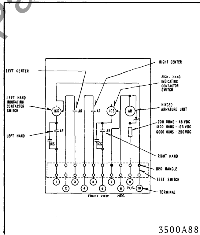
Fig. 6. Internal schematic of the Type AR Relay - High Threshold - with 4 make contacts and 2 ICS units in FT-11 case.
