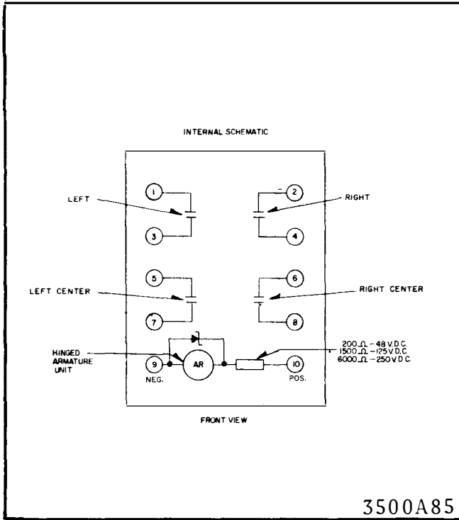
Fig. 3. Internal schematic of the Type AR Relay - High Threshold - with 4 make contacts in front connected molded case.
