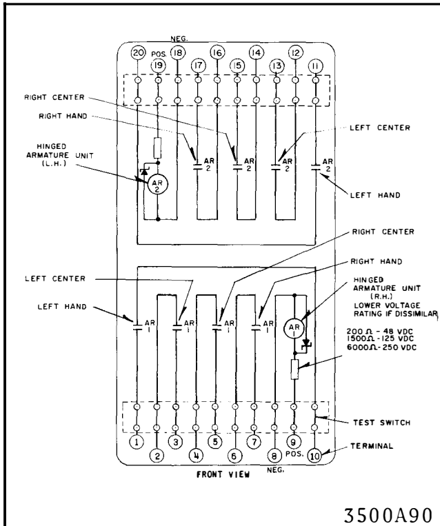
Fig. 7. Internal schematic of the Type AR Relay - High Threshold - double unit with 8 make contacts in FT-22 case.
