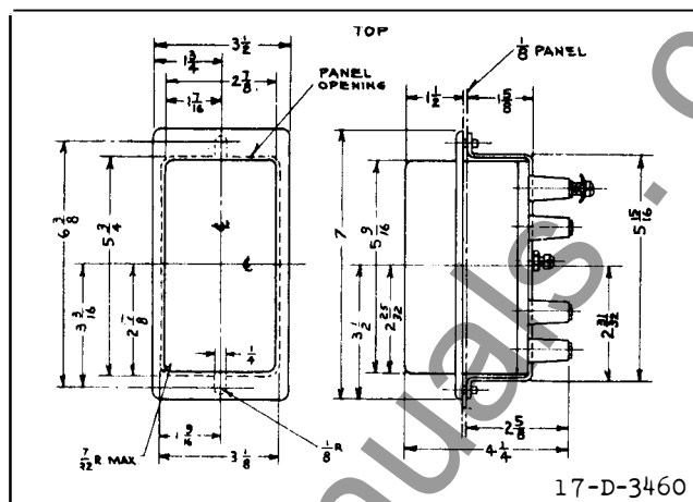
Fig. 6 Outline and Drilling Plan for the Semi-flush Case for the Type SG Relay. For Reference Only.
