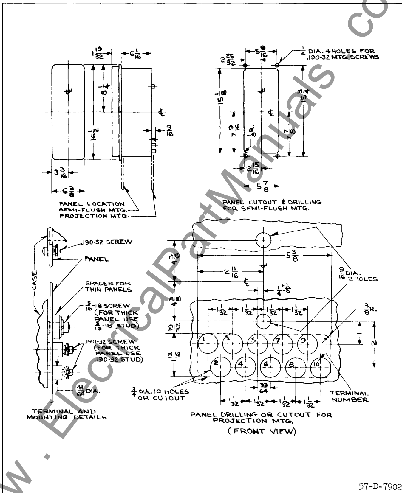
Fig. 9. Outline and Drilling Plan for the HLF Relay in the FT31 Case.
