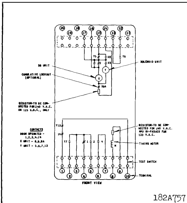
Fig. 2. Internal Schematic of the RC Relay, Without Z Unit, in Type FT32 Case.
