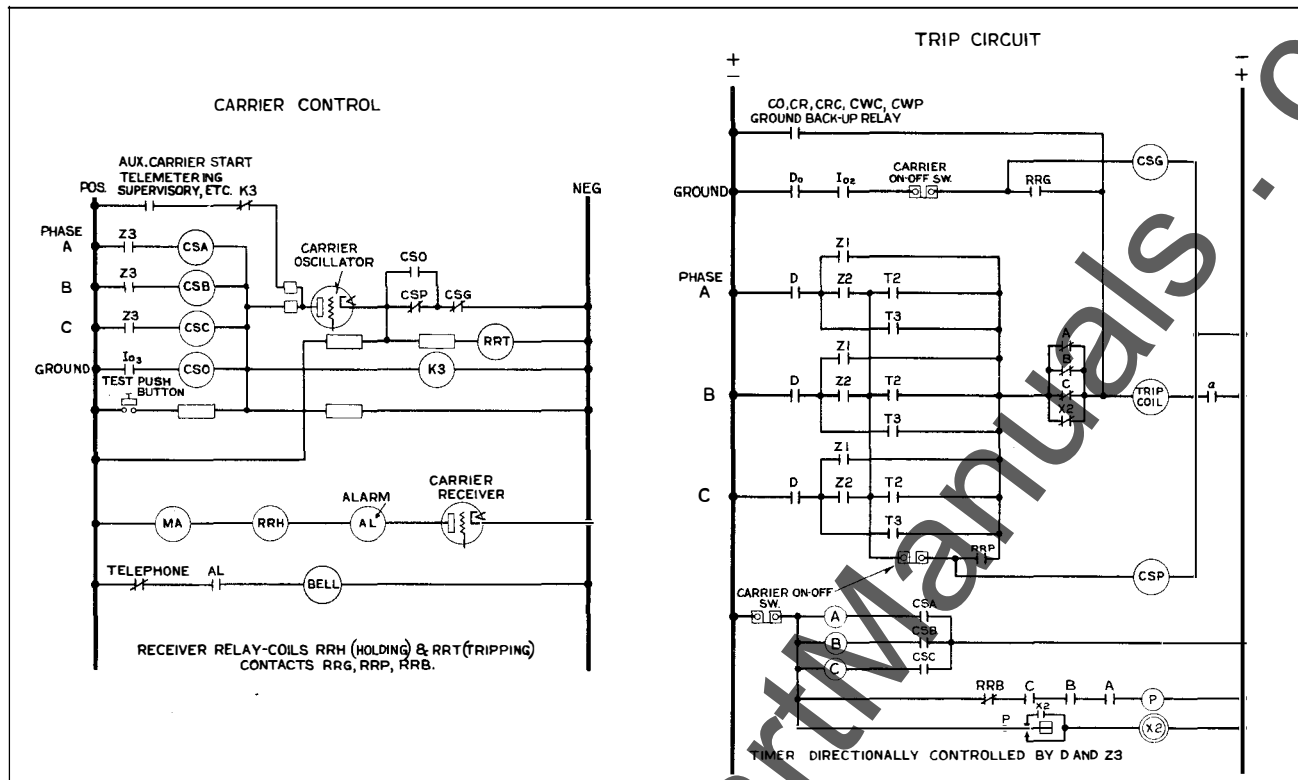
Fig. 1—Simplified D-C Schematic of the Carrier Relaying Scheme.
