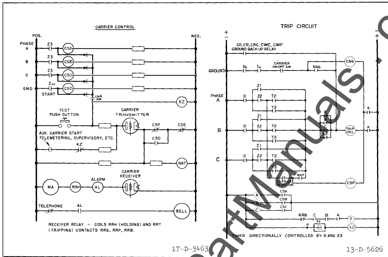
Fig. 1—Simplified D-C Schematic Of The Carrier Relaying Scheme.
