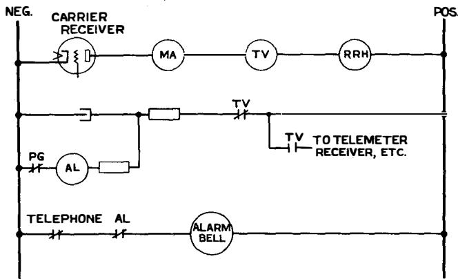
Figure 3 Time Delay Circuit For the Carrier Alarm When Using the Carrier Channel For Telemetry or Supervisory.
