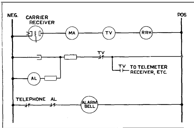
Fig. 3—Time Delay Circuit For the Carrier Alarm When Using the Carrier Channel For Telemetry or Supervisory.
