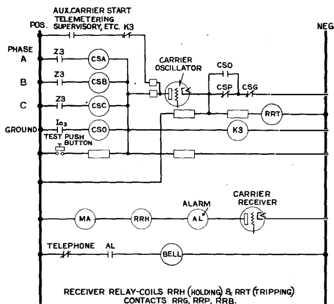
Figure 1 Simplified D-C Schematic of the Carrier Relaying Scheme.
