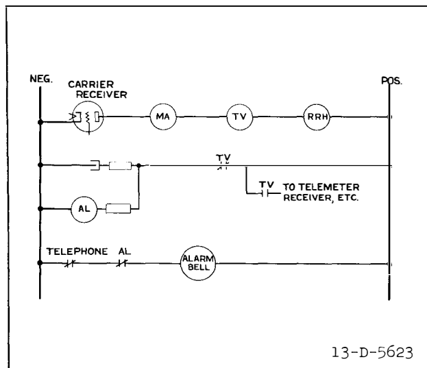
Fig. 3—Time Delay Circuit For The Carrier Alarm When Using The Carrier Channel For Telemetry Or Supervisory.
