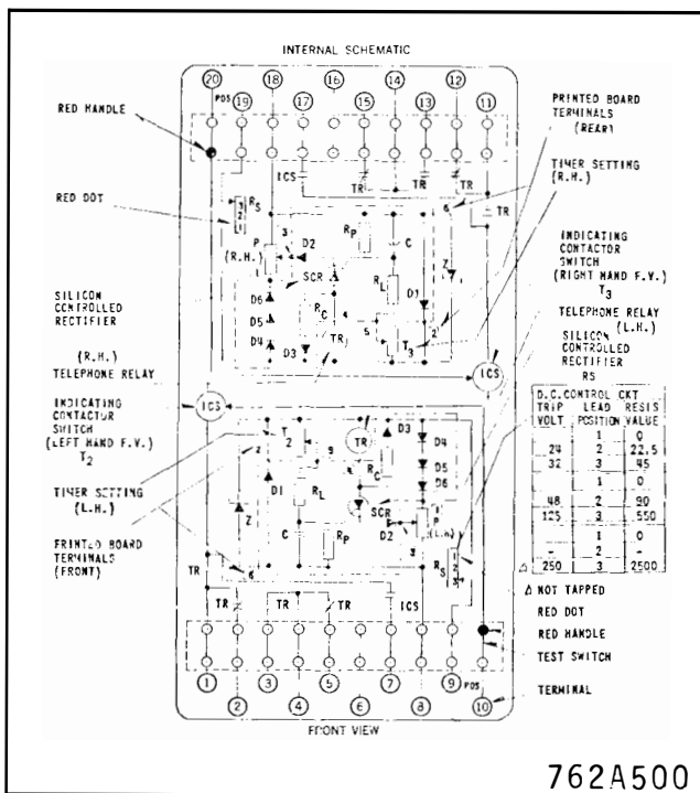
Fig. 2. Internal Schematic of Type TD-52 Relay with Single Trip 0.2/2.0 Ampere ICS Units (Relay with Single Trip 1.0 Ampere ICS Units has Identical Wiring Except the ICS Coils are not Tapped on Terminals 10 and 20, 849A417).
