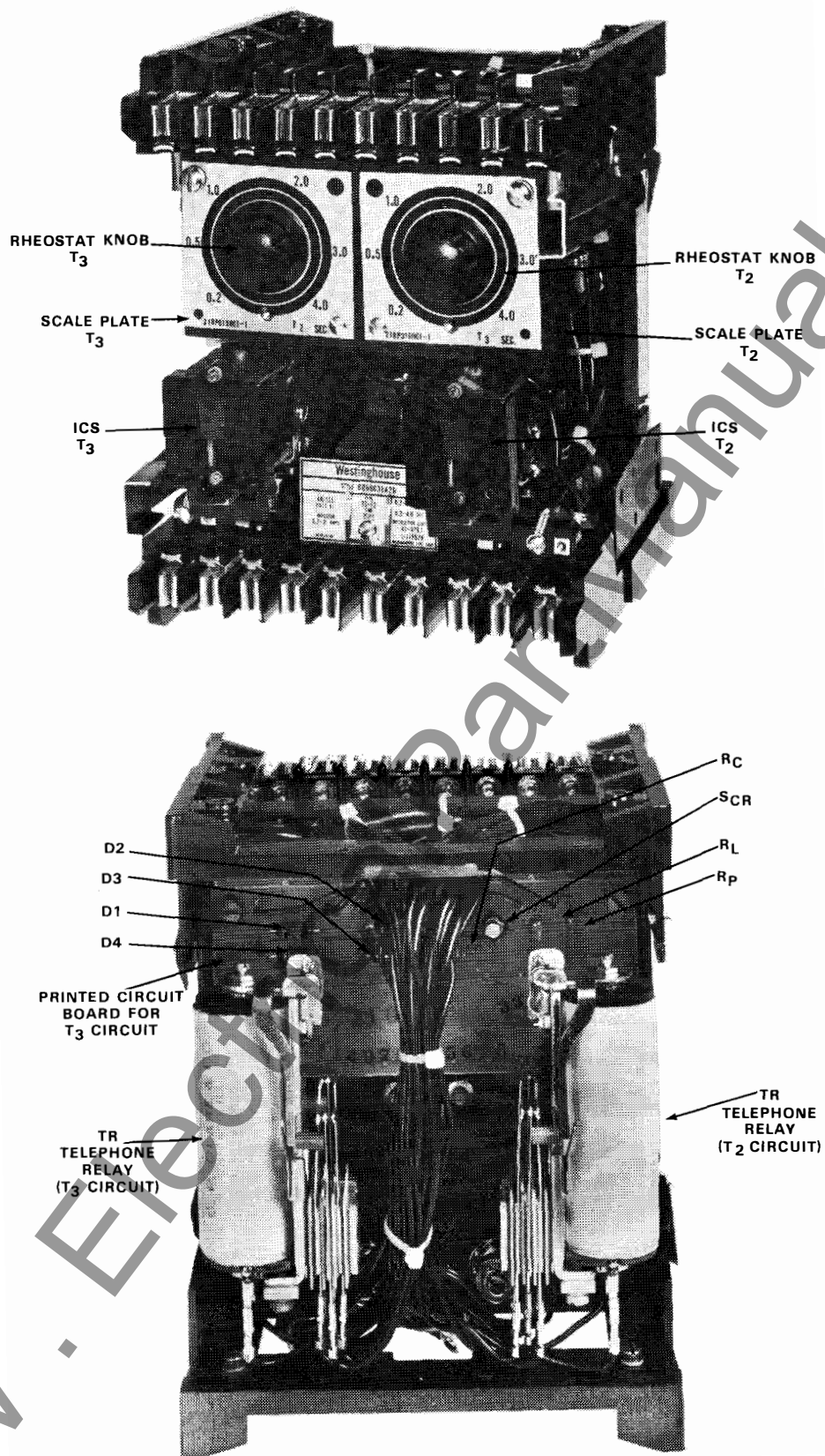
Fig. 1. Type TD-52 Relay Without Case.
