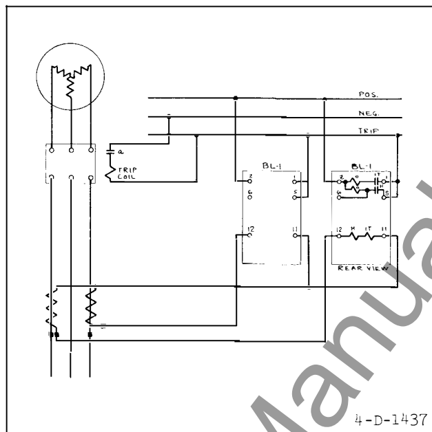
Fig. 12—Typical Diagram of External Connections for the Type BL-1 Relay used to Protect a Machine against Excessive Temperatures when Running Three-Phase or Single-Phase.
