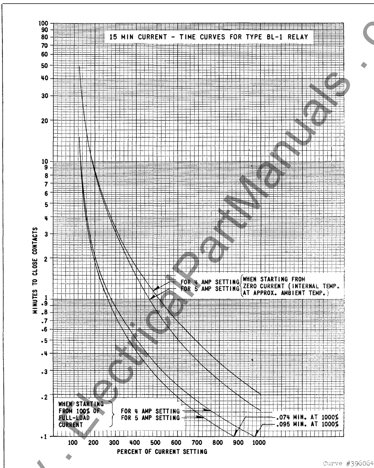
Fig. 9—Current-Time Curves for Special Applications of the Type BL-1 Relay Covering Range of Full-Load Currents from 4.0 to 5.0 Amperes. Contact Settings Determined by Test for 15-Minute Delay with 125% Load Occurring after Moving Contact reaches Final Position for Steady Full Load. Shorting Link Closed.
