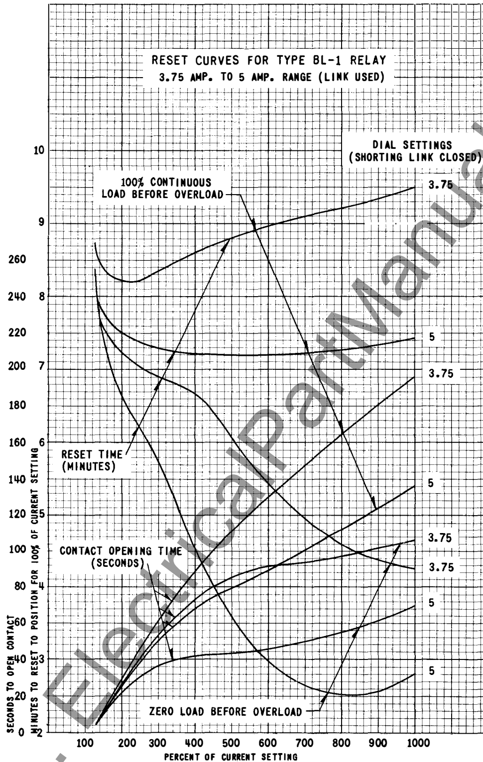
Fig. 11—Contact-Opening and Reset Time Curves for the Type BL-1 Relay for Full-Load Settings of 3.75 to 5.0 Amperes as marked on Dial. Shorting Link Closed.
