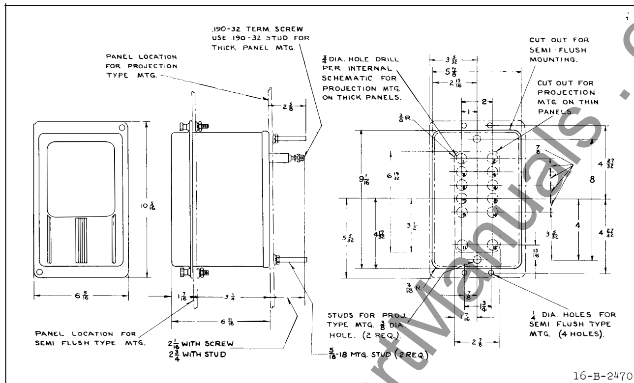
Fig. 14—Outline and Drilling Plan for the S-10 Semi-Flush or Projection Type FT Flexitest Case. (See the Internal Schematic for the Terminals Supplied.) For Reference Only.
