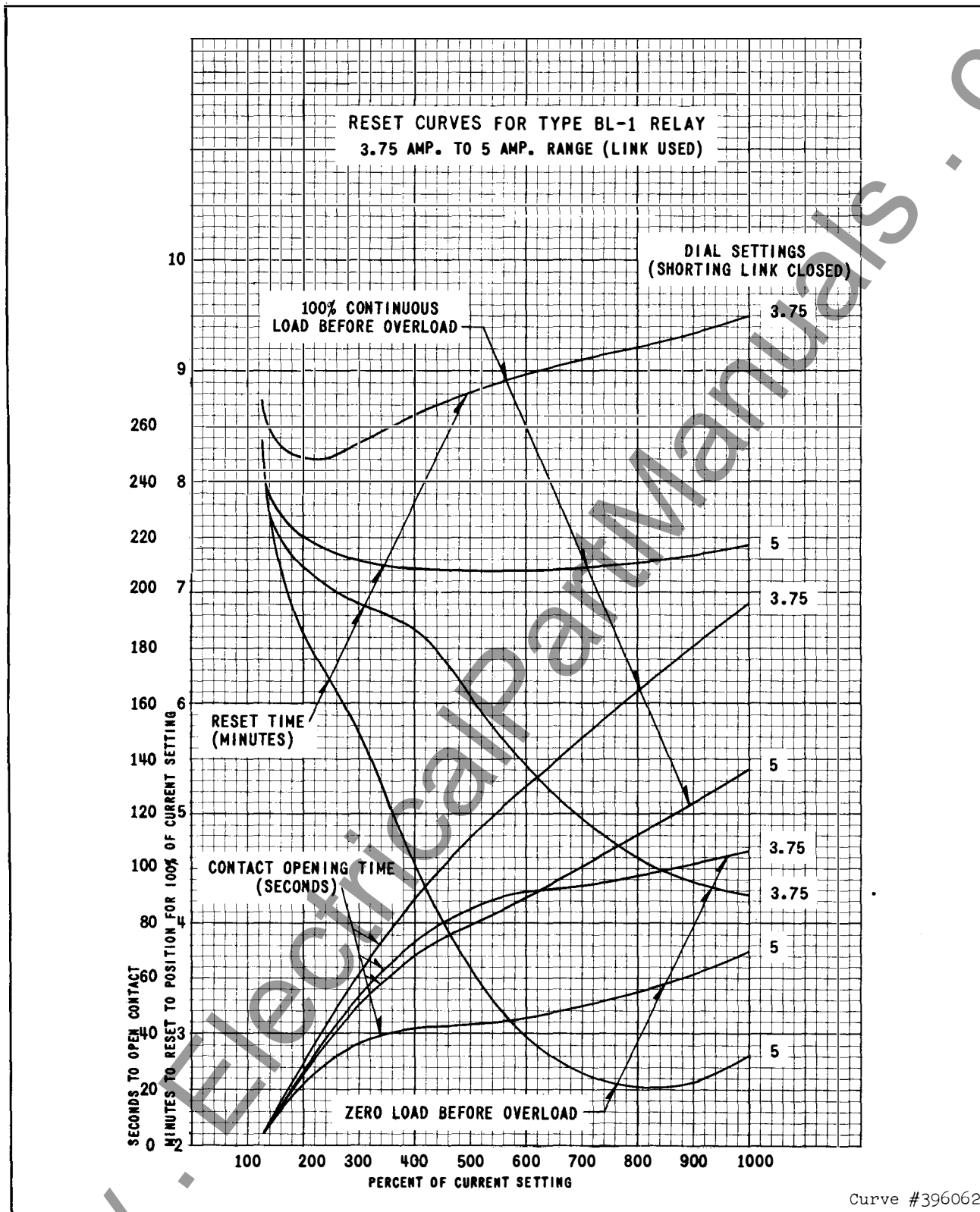
Fig. 11—Contact-Opening and Reset Time Curves for the Type BL-1 Relay for Full-Load Settings of 3.75 to 5.0 Amperes as marked on Dial. Shorting Link Closed.
