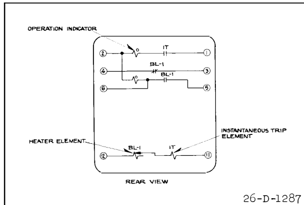
Fig. 1—Internal Schematic of the Single Element Type BL-1 Relay with Front and Back Contacts in the Standard Case. The Relay with Front Contacts only has Terminals 3 and 4 Omitted.
