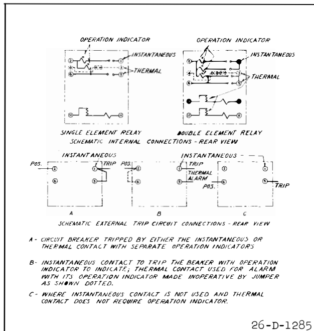
Fig. 5—Schematic Trip Circuit Connections for Various Applications of Single and Double Element Type BL-1 Relays in the Standard Cases.
