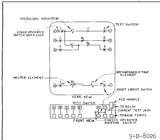
Fig. 3—Internal Schematic of the Single Element Relay with Front and Back Contacts in the Type FT Case. The Relay with Front Contacts Only has Terminals 3 and 4 and Associated Circuits Omitted.
