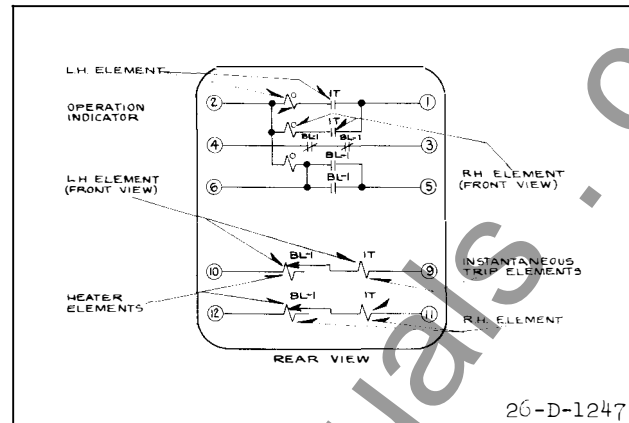
Fig. 2—Internal Schematic of the Double Element Relay with Front and Back Contacts in the Standard Case. The Relay with Front Contacts Only has Terminals 3 and 4 and Associated Circuits Omitted.
