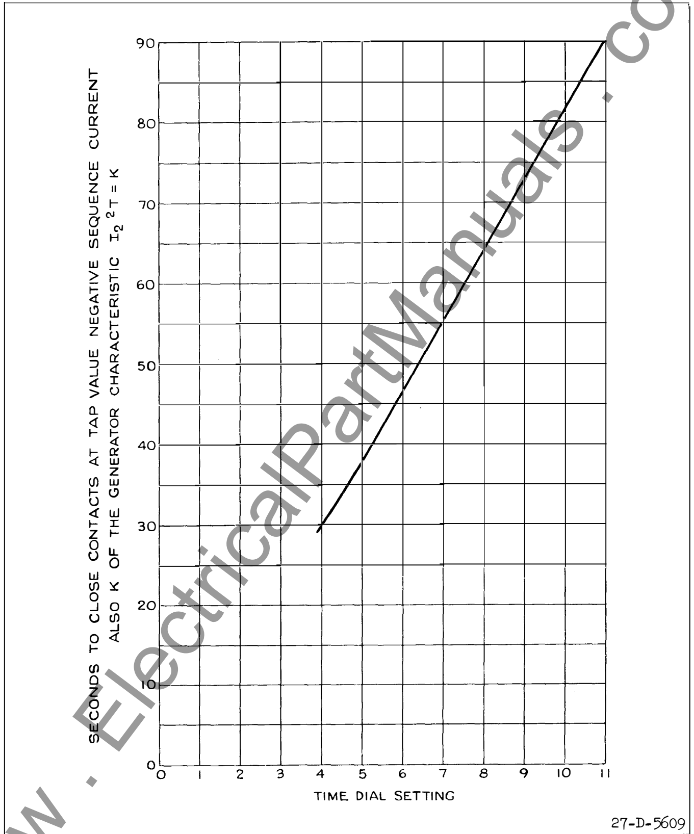
Fig. 4. Required COQ Time Dial Setting Versus Generator Constant.
