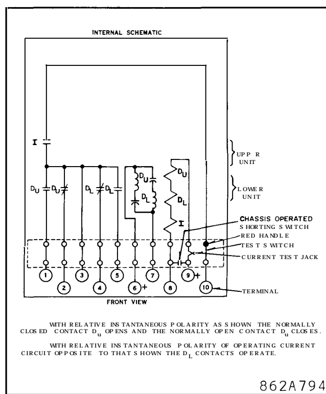
Fig. 2 Internal Schematic (with IT Unit) (.02 to 1 amp range)
