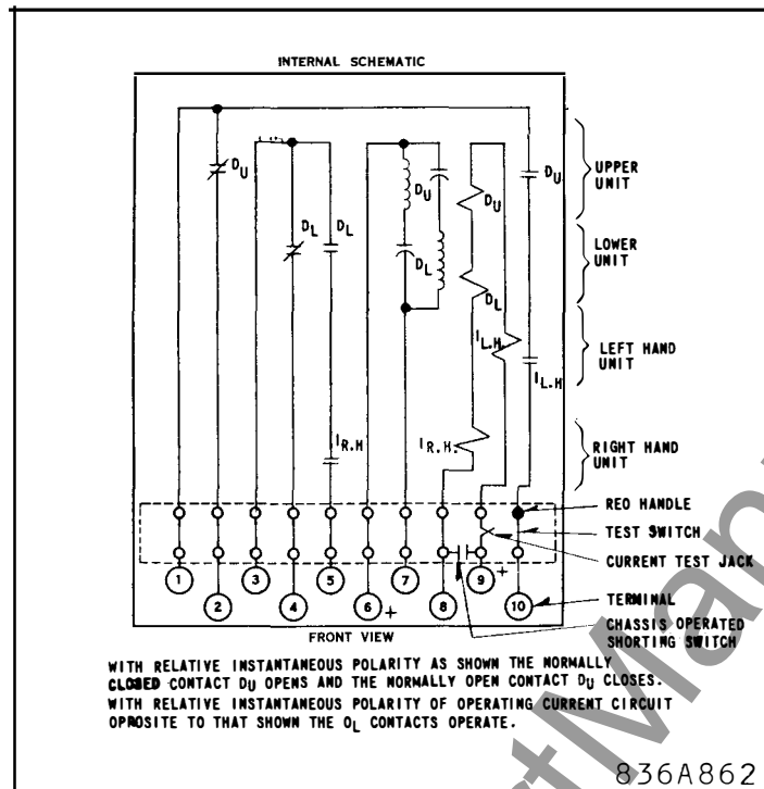
Fig. 2a Internal Schematic (with IT Units) (.5 to 2 amp range)
