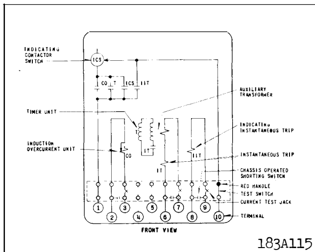
Fig. 1. Internal Schematic of the Type CO-4 Relay in the Type FT21 Case.
