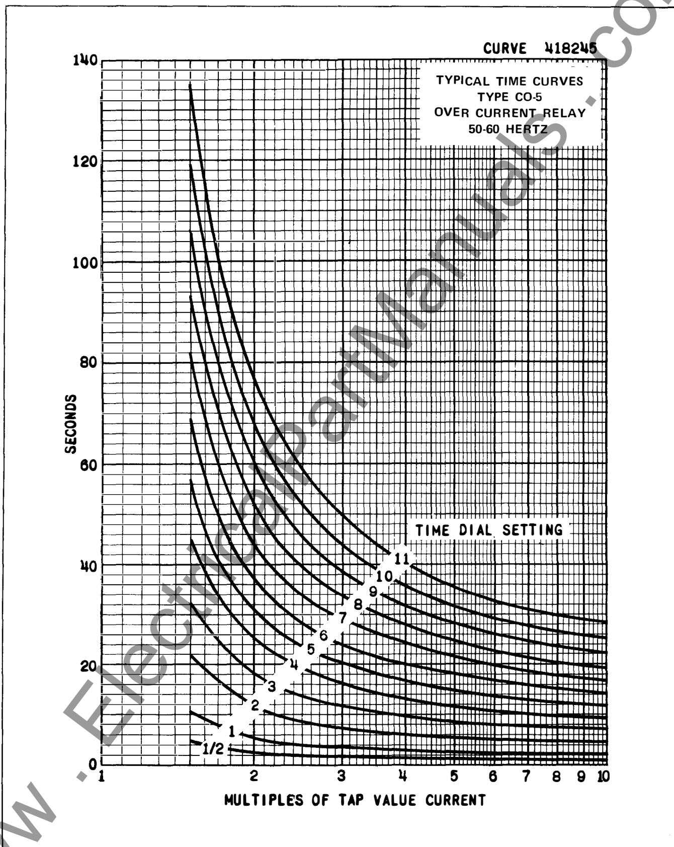
Fig. 2. Typical Time Curves of the Overcurrent Unit.
