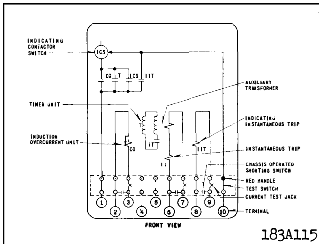
Fig. 1. Internal Schematic of the Type CO-4 Relay in the Type FT21 Case.
