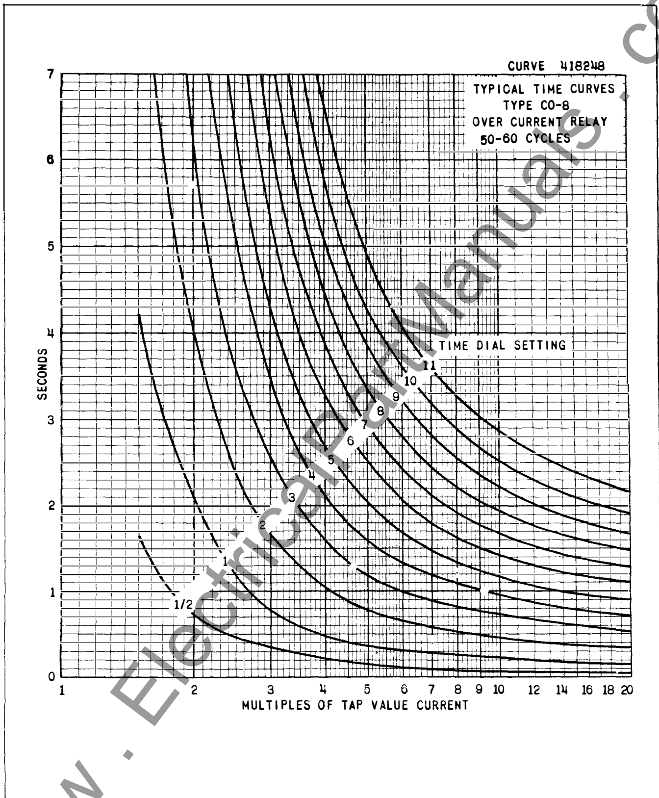
Fig. 7. Typical Time Curves of the Type CO-8 Relay.
