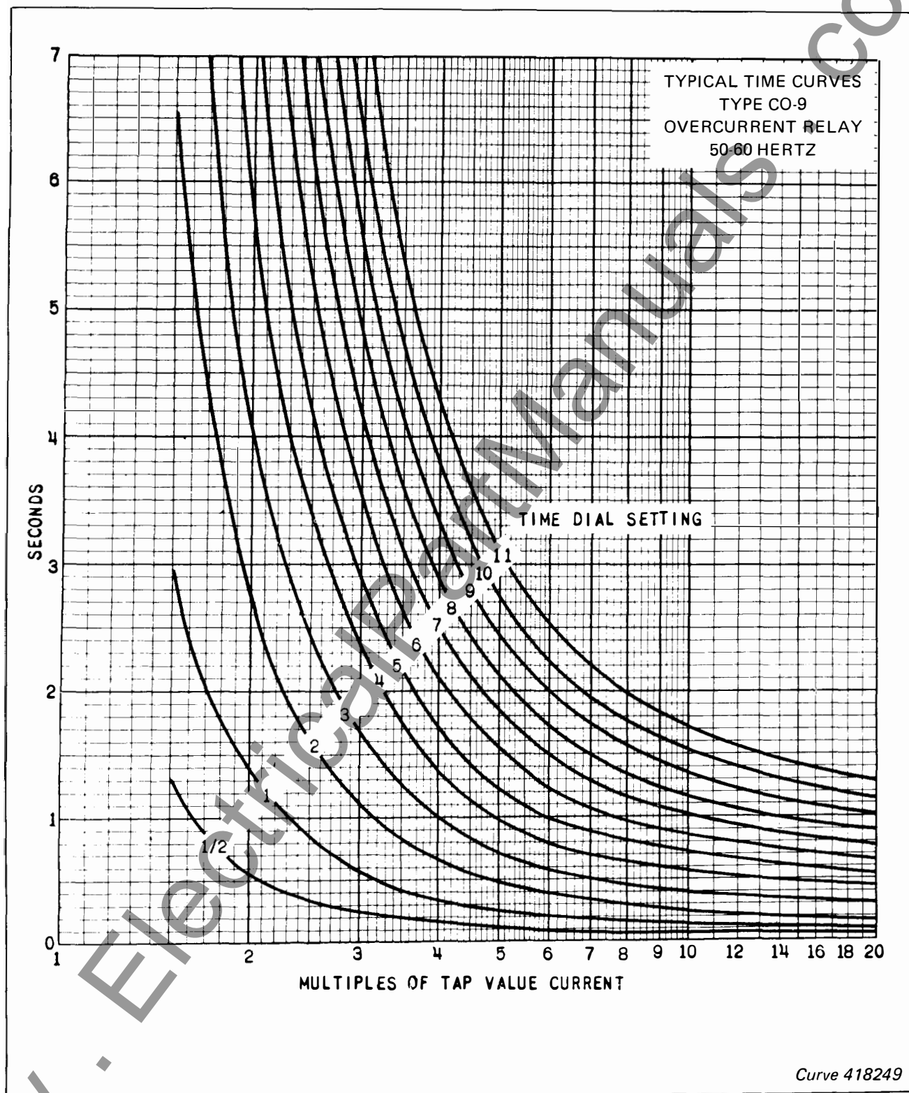
Fig. 8. Typical Time Curve of the Type CO-9 Relay
