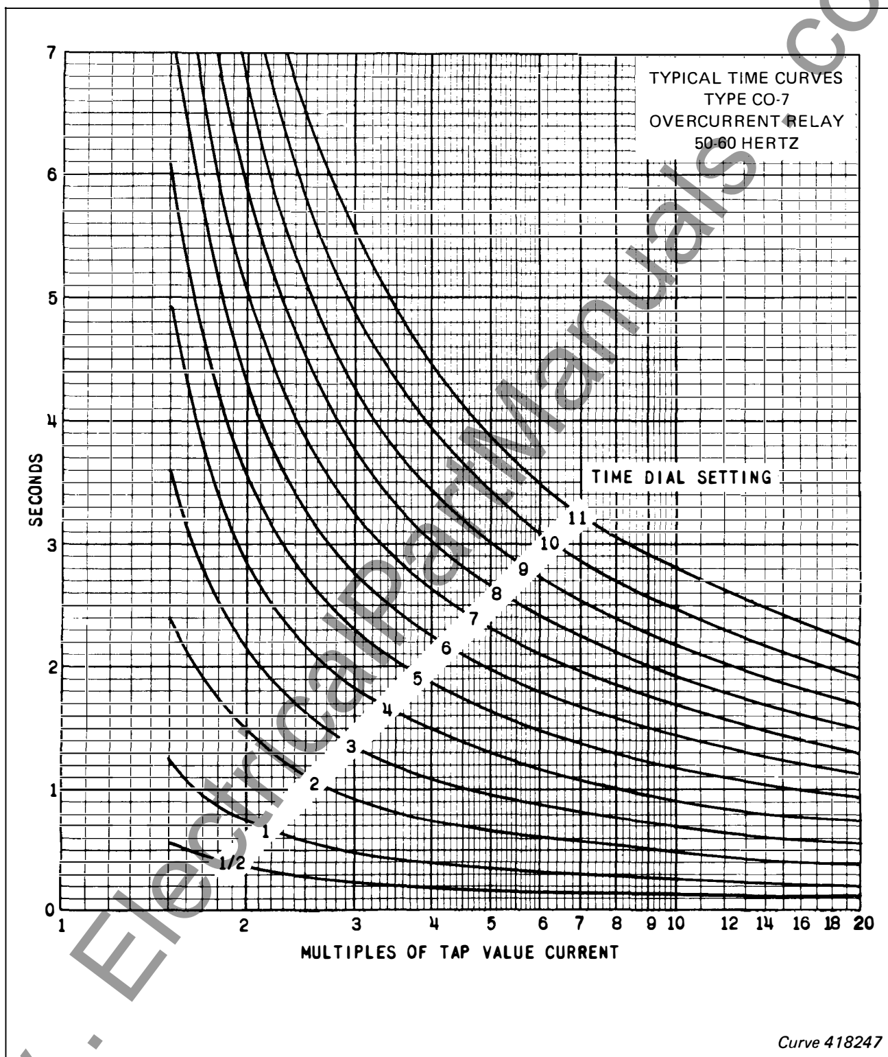
Fig. 6. Typical Time Curve of the Type CO-7 Relay
