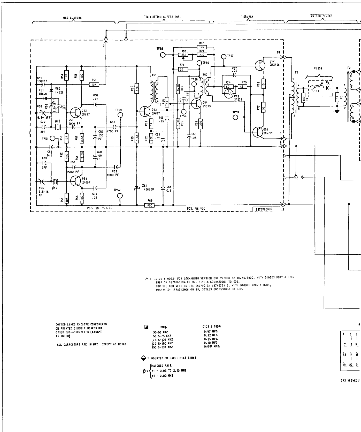
Fig. 2 - Internal Schematic of Type TCF Transmitter :
