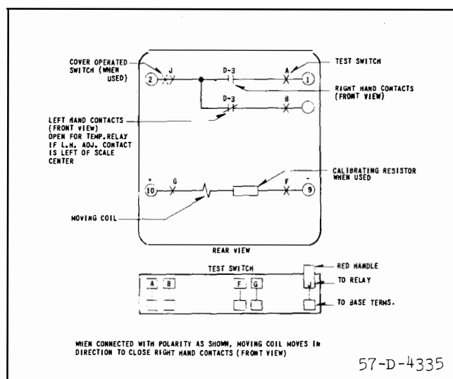
Fig. 2. Internal Connections of the Type DT-3 Relay in the Type FT Case. Omit Test Switches for the Relay in the Standard Case.
