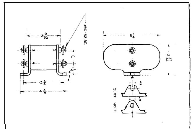
Fig. 6. Outline and Drilling Plan for the Two-Spool Resistor Cage Used with the Type DT-3 Temperature Relay. For Reference Only.
