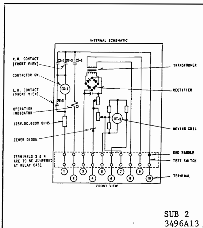
Fig. 6. Internal Schematic of the DT-3 Relay for use with 120 ohm 0°C nickel RTD with operation indicator.
