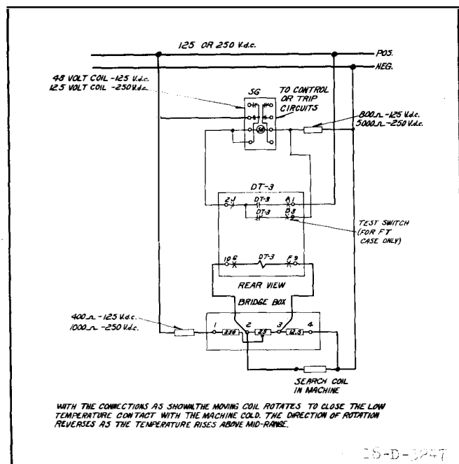
Fig. 3. External Connections for Thermal Protection of Electrical Equipment, using the type DT-3 Temperature Relay in Either the FT Case or the Stand Case.
