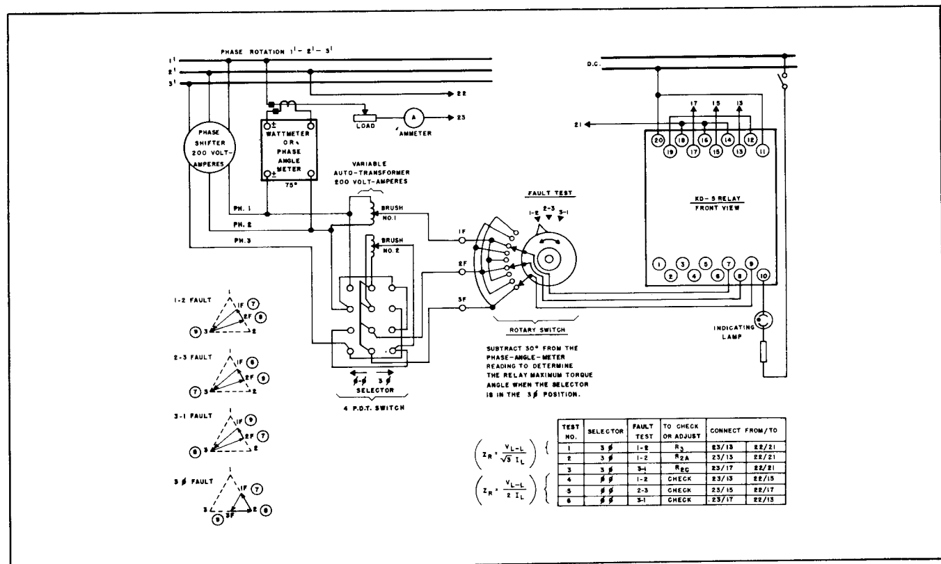
Fig. 17 Test Connections for Type KD-5 Relay.
