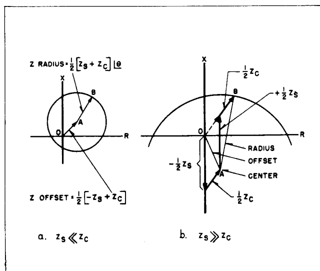
Fig. 7 Impedance Circles for Phase-to-Phase Unit in the Type KD-5 Relay.
