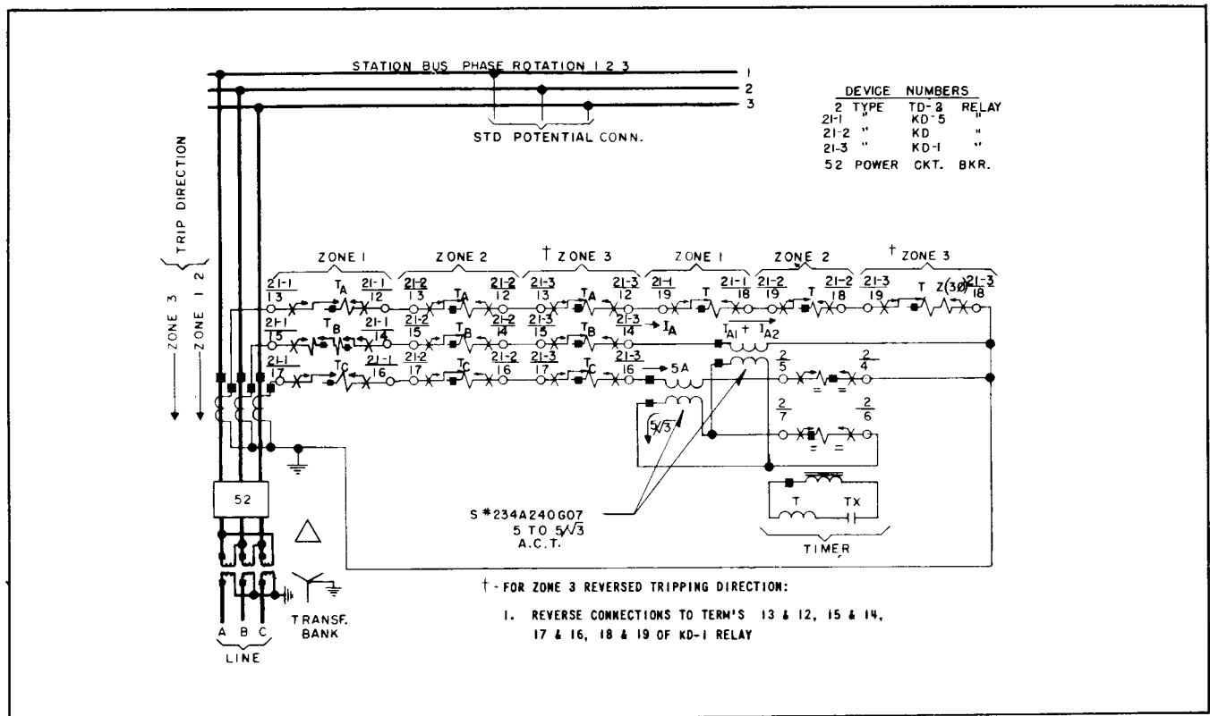
Fig. 16 A.C. External Schematic of Type KD-5 KD and KD-1 Relays with Type TD-2 Timing Relay-Wye-Delta Bank Termination with Delta on Relay Side.
