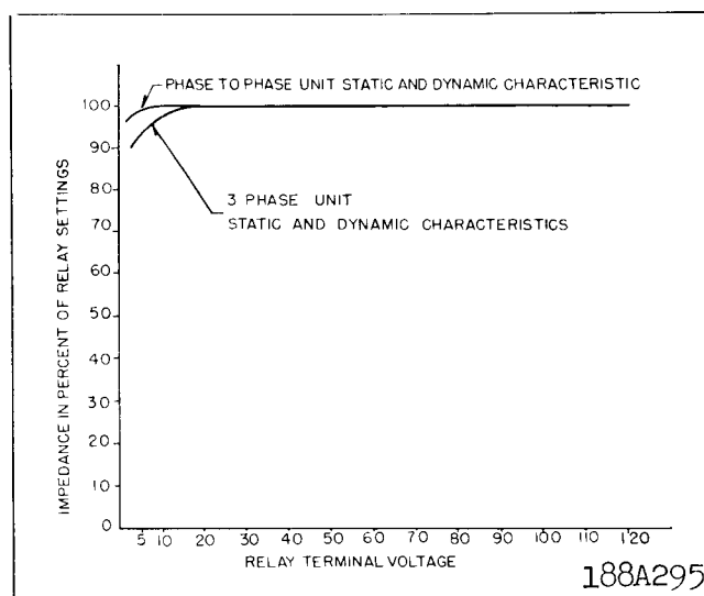
Fig. 8 Impedance Curves for Type KD-5 Relay.
