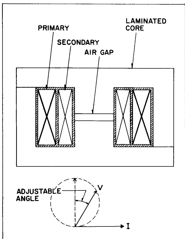
Fig. 2 Compensator Construction
