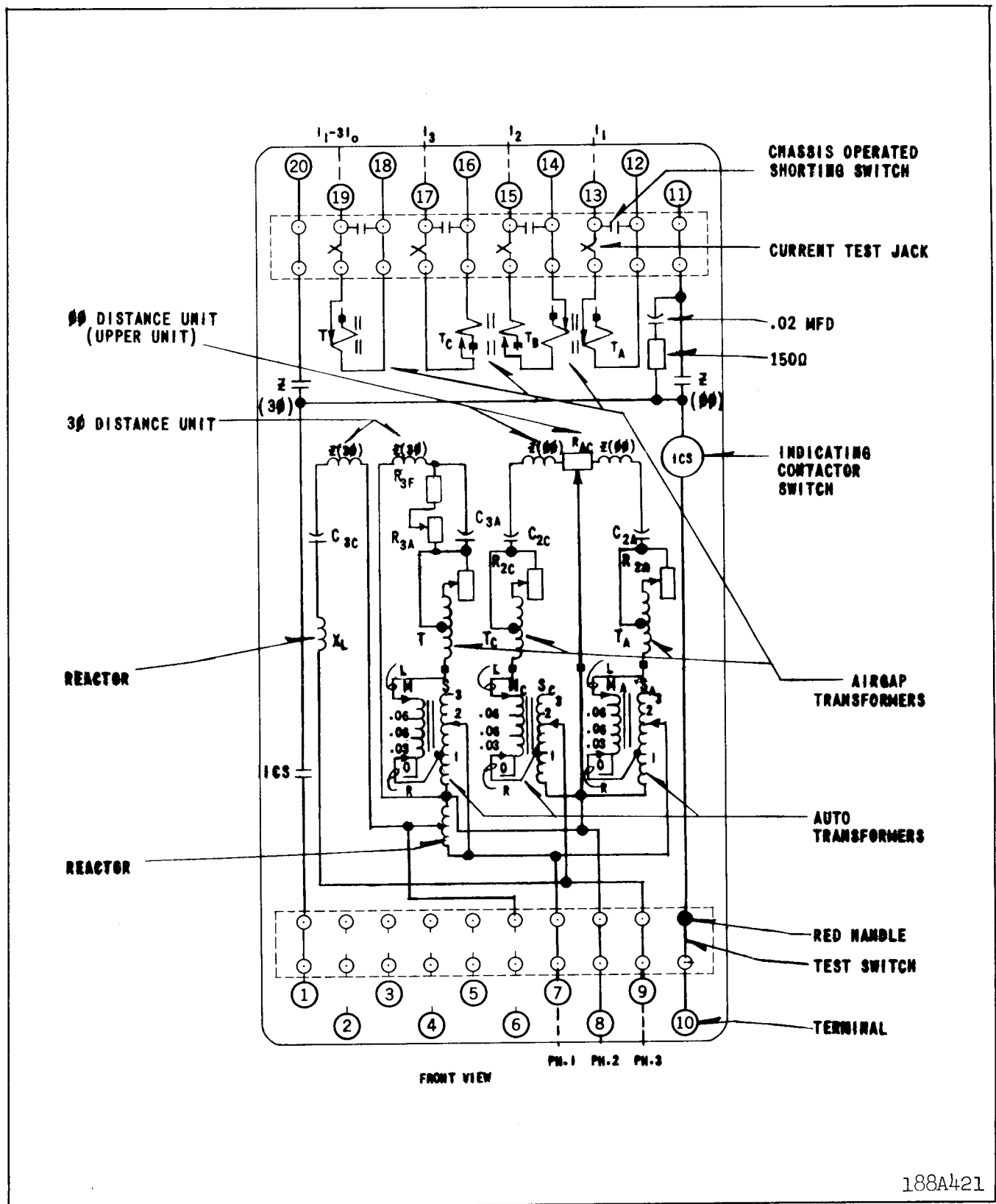
Fig. 4 Internal Schematic of Type KD-5 Relay with 1.0 ampere I.C.S. in the type FT42 case. (Relay with 0.2/2.0 ampere I.C.S. unit has identical wiring except that the I.C.S. coil is tapped on terminal 10 (188A426).
