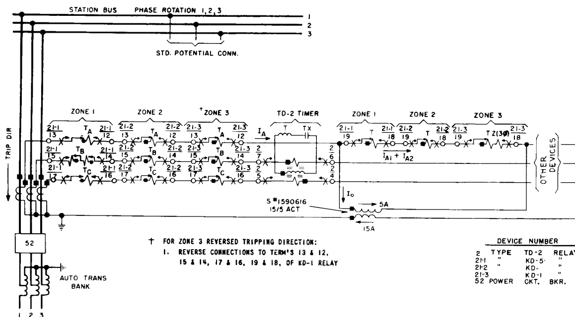
Fig. 14 A.C. External Schematic of Type KD-5 KD and KD-1 Relays with Type TD-2 Timing Relay-Auto-transformer Termination.
