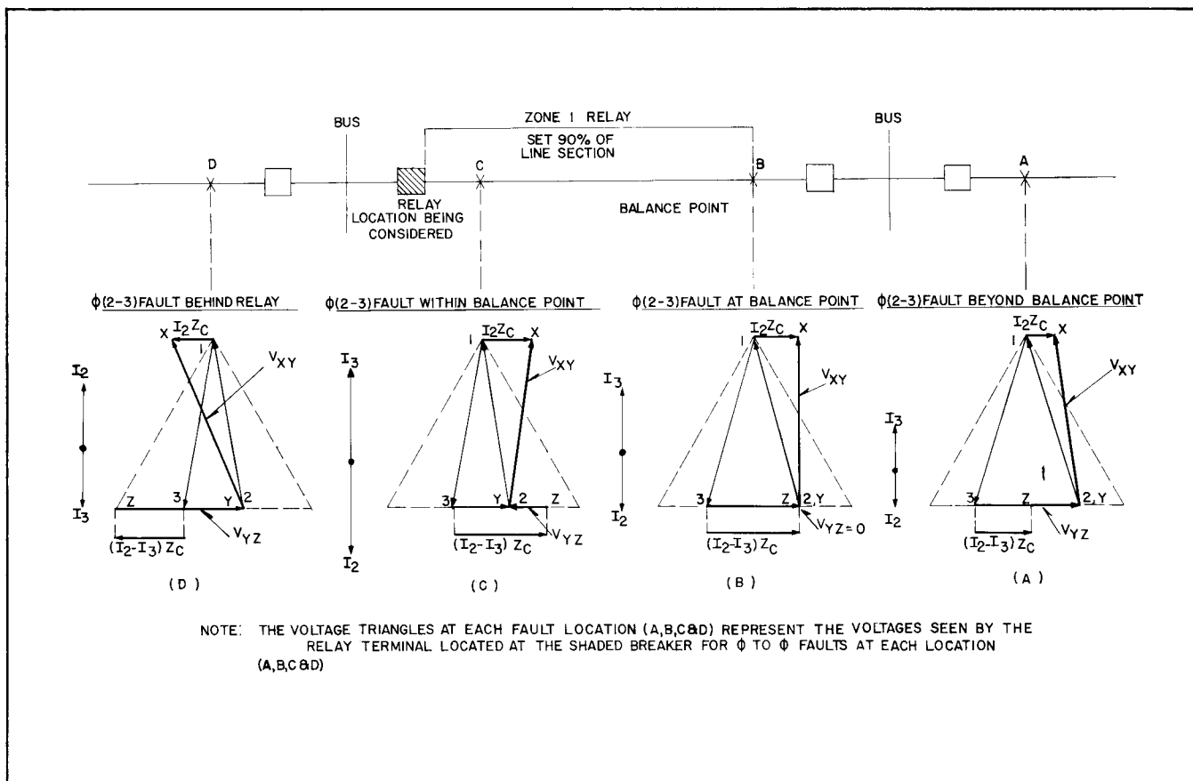
Fig. 6 Voltage and Current Conditions for the Phase-to-Phase Unit at the Shaded Breaker for \phi (2-3) Faults at various Locations.
