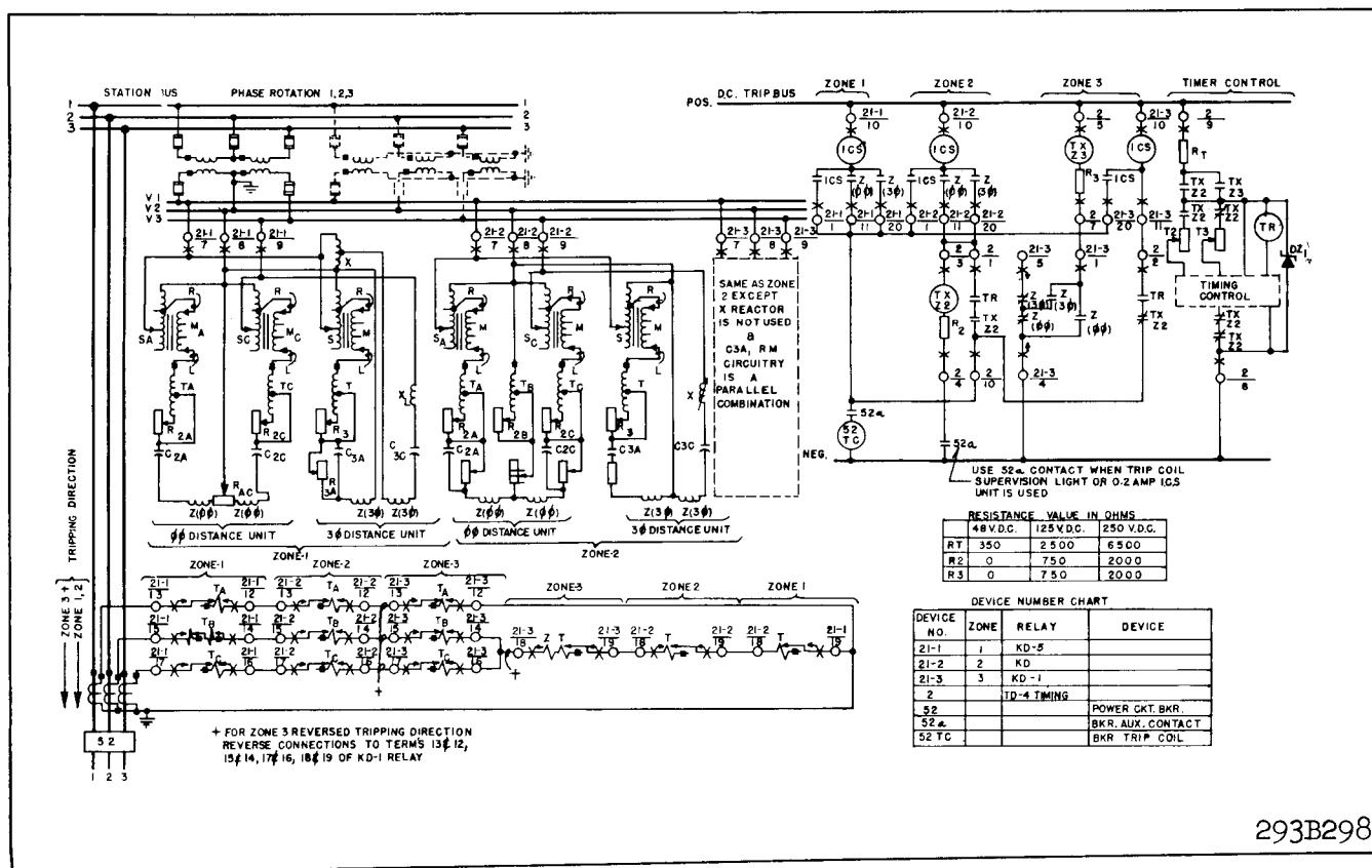
Fig. 13 External Schematic of Type KD-5, KD and KD-1 Relays with Type TD-4 Timing Relay.
