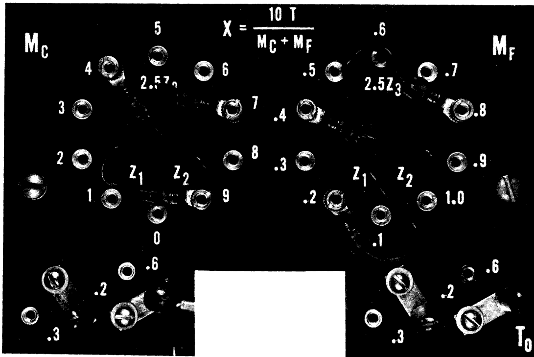
* Fig. 4. Tap Plate
