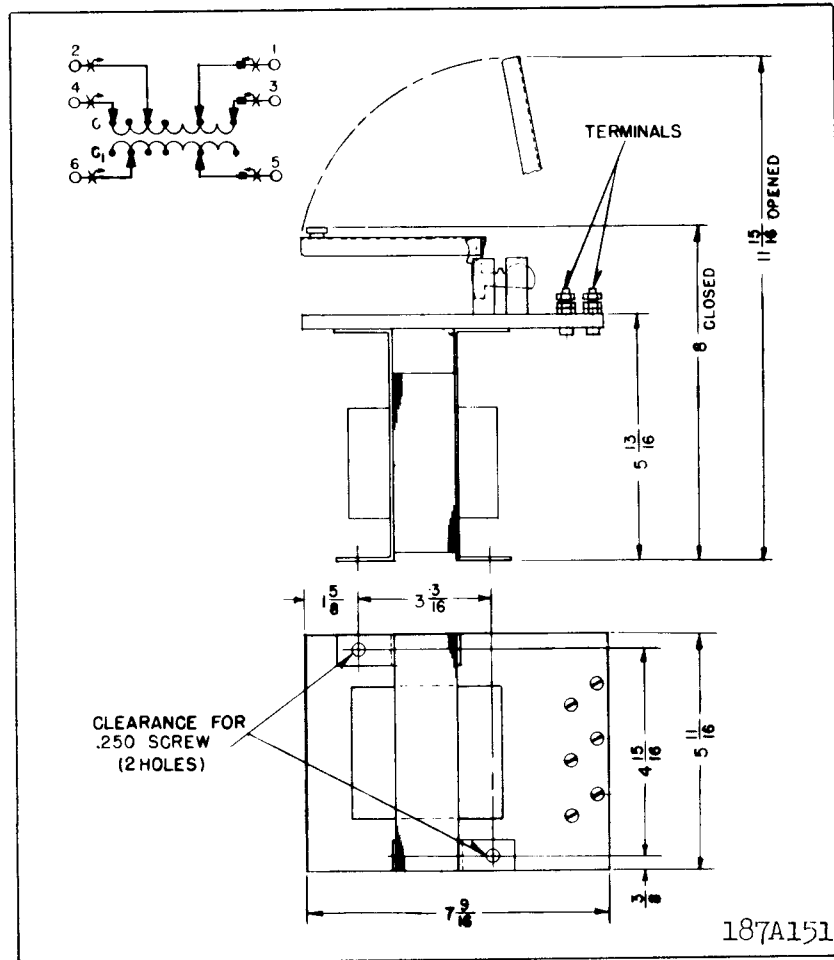
Fig. 12. Outline-Drilling Plan for Type 1K Auxiliary CT.
