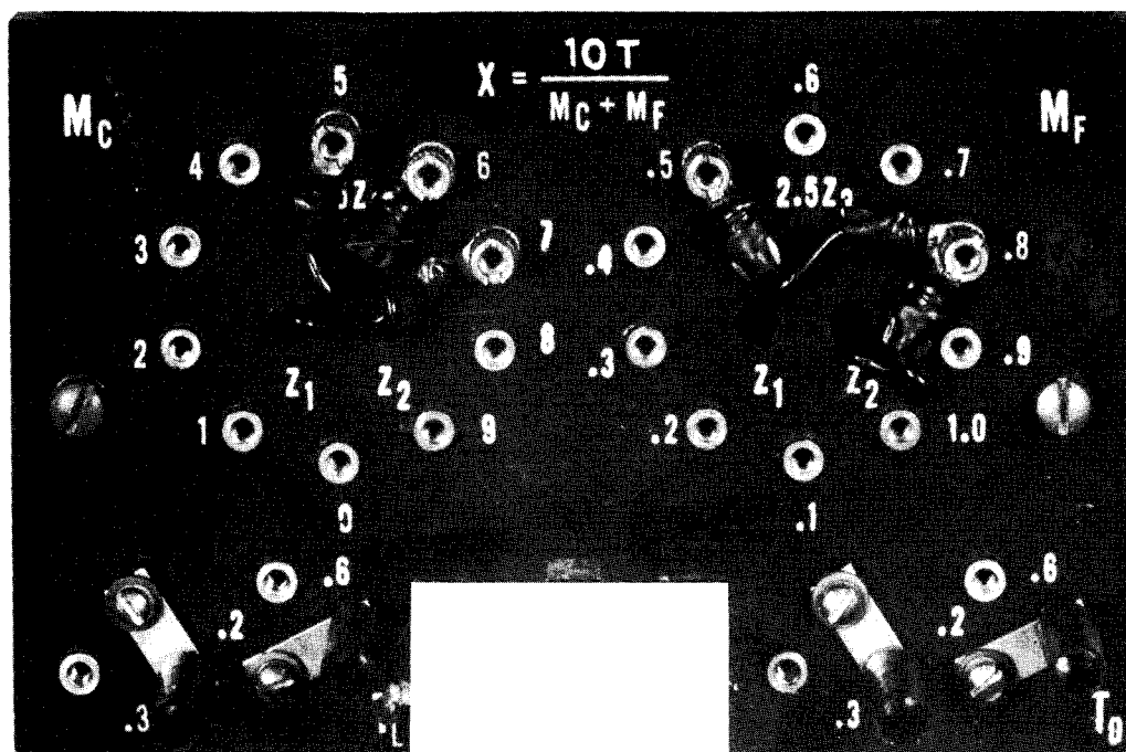
Fig. 4. Tap Plate
