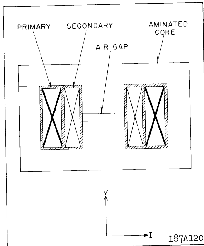
Fig. 3. Compensator Construction.
