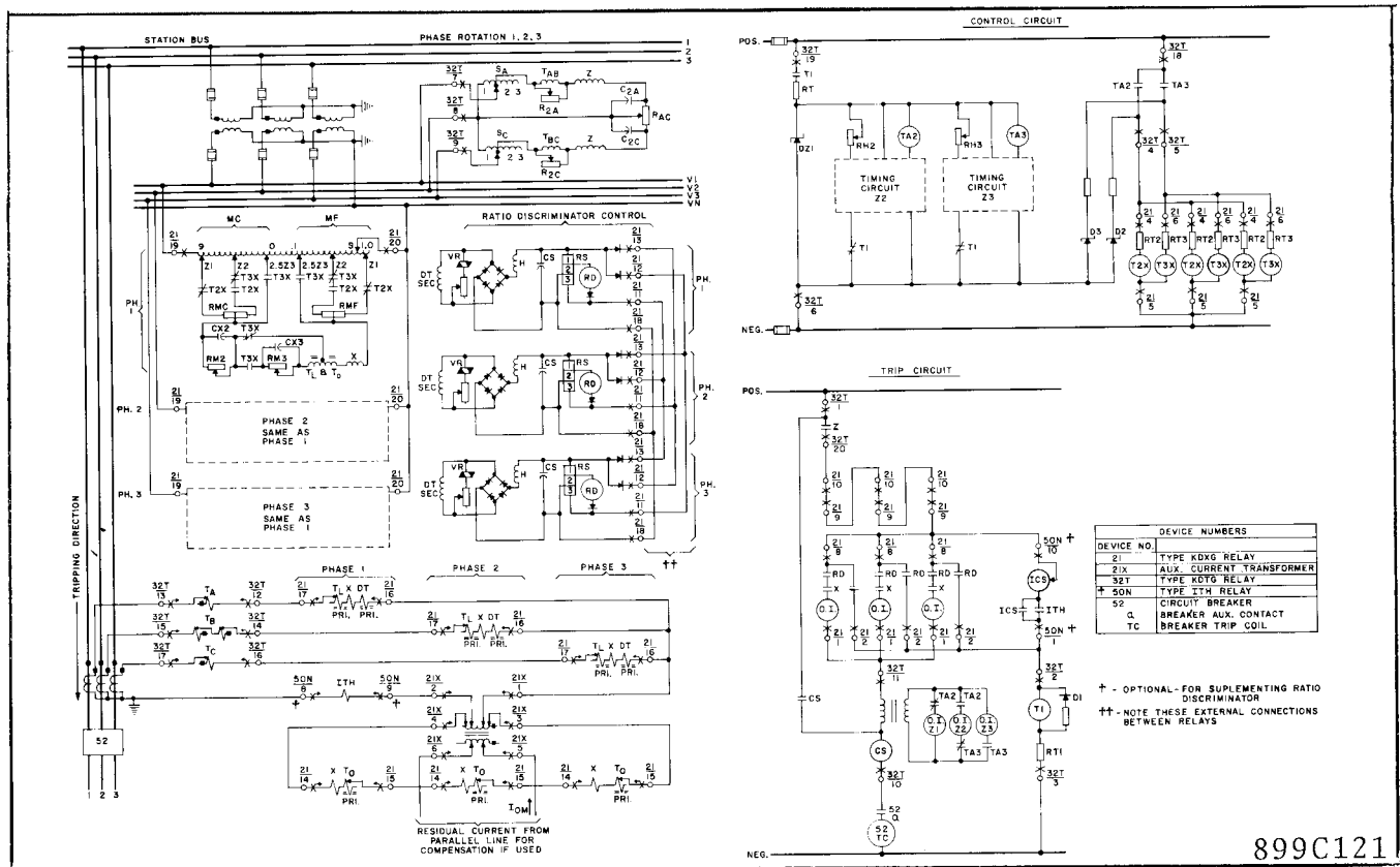
* Fig. 14. External Schematic for Type KDXG and KDTG Relays
