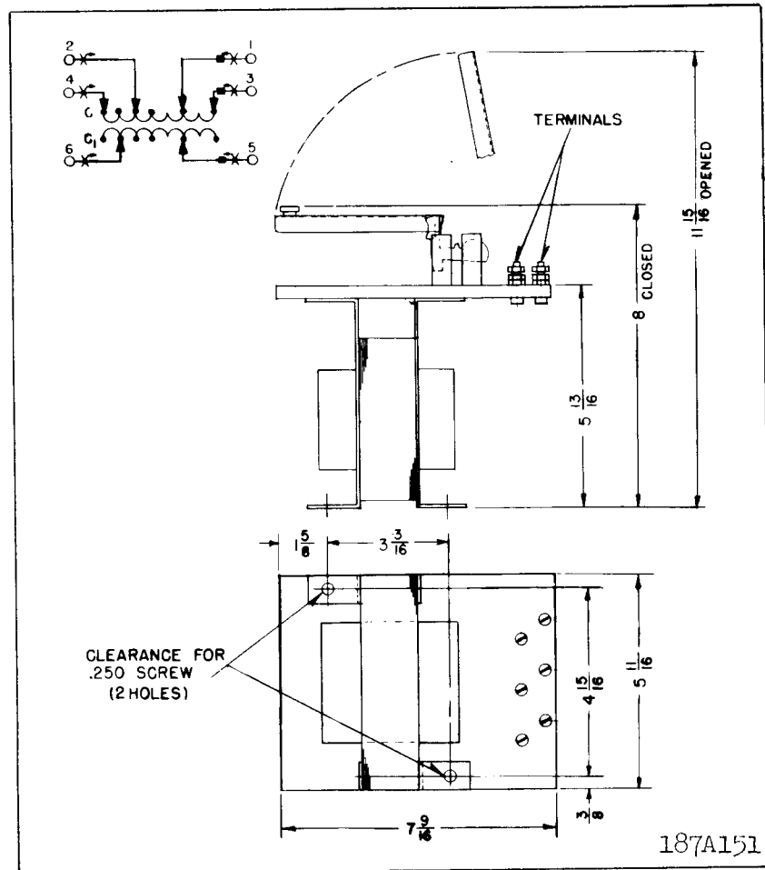
Fig. 12. Outline-Drilling Plan for Type 1K Auxiliary CT.
