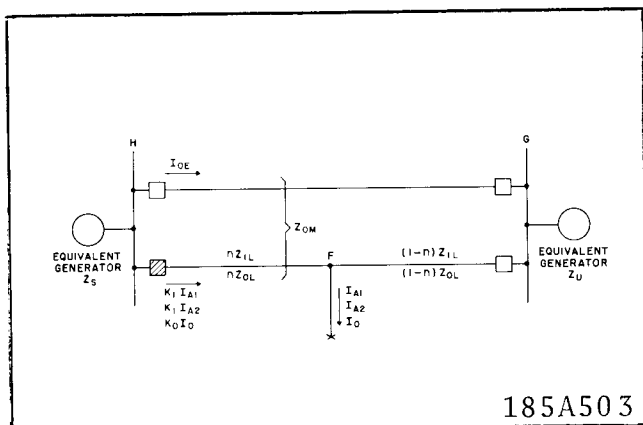
Fig. 7. General System Used for Describing Type KDXG Relay Operations
