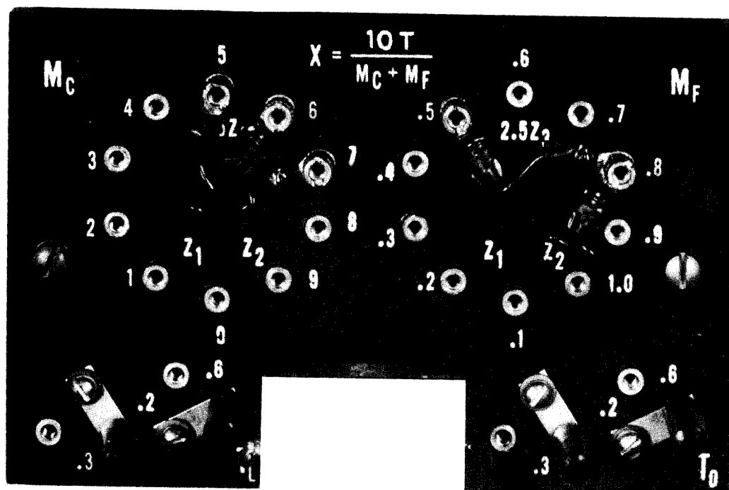
Fig. 4. Tap Plate
