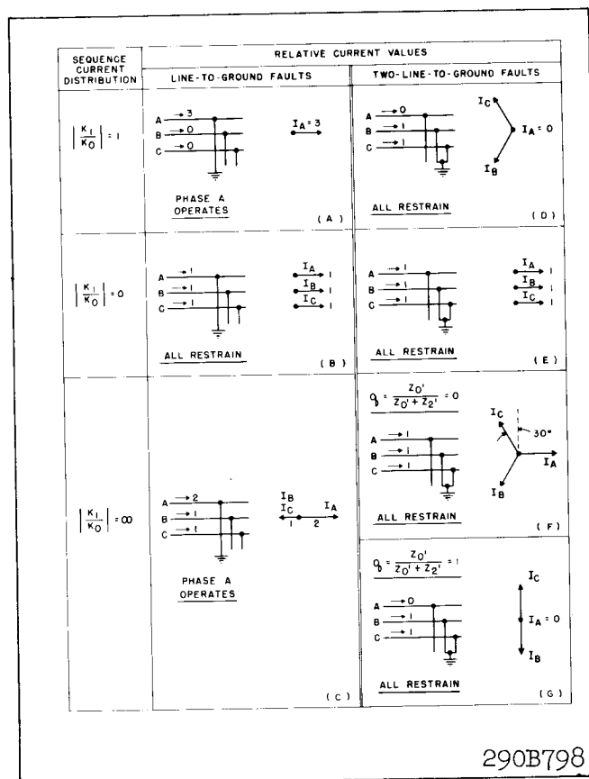
Fig. 8. Response of Ratio Discriminator to Ground Faults, Assuming All Impedances in Phase.
