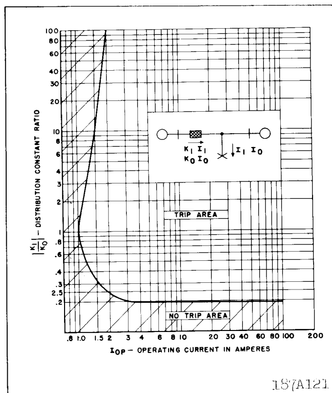
Fig. 9. Typical Operating Characteristics of the Ratio Discriminator as a Function of Current Distribution Factor Ratio and Operating Current.
