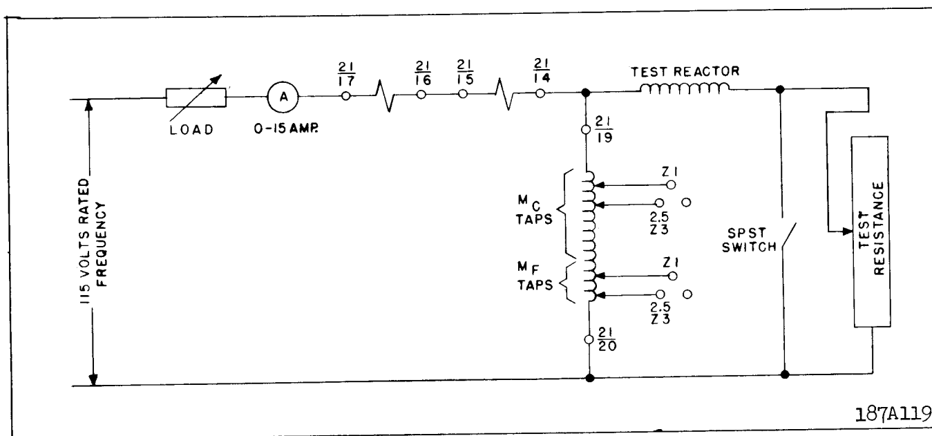
Fig. 14. Circuit For Reactance Unit Phase Angle Adjustment
