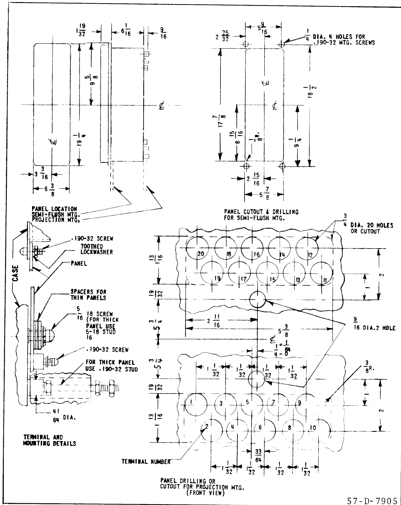
Fig. 17. Outline - Drilling Plan for Type KDXG - Relay in FT42 Case.
