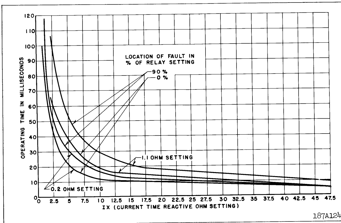
Fig. 15. Typical Operating Time Curves of the Reactance Unit.
