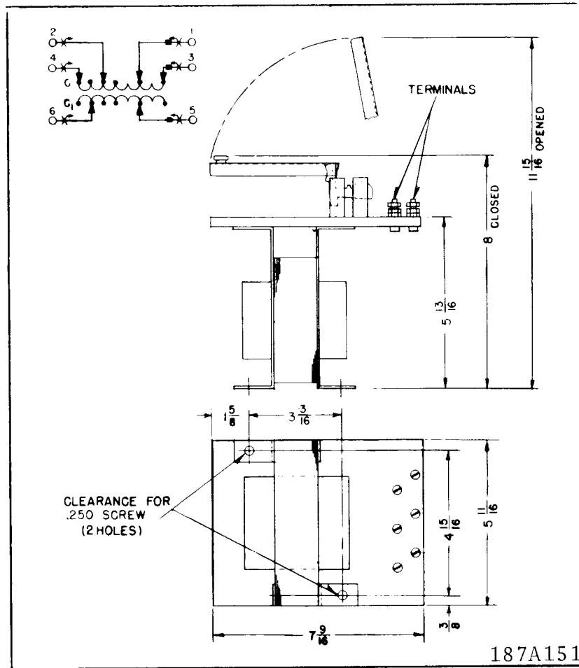
Fig. 12. Outline - Drilling Plan for Type IK Auxiliary CT.
