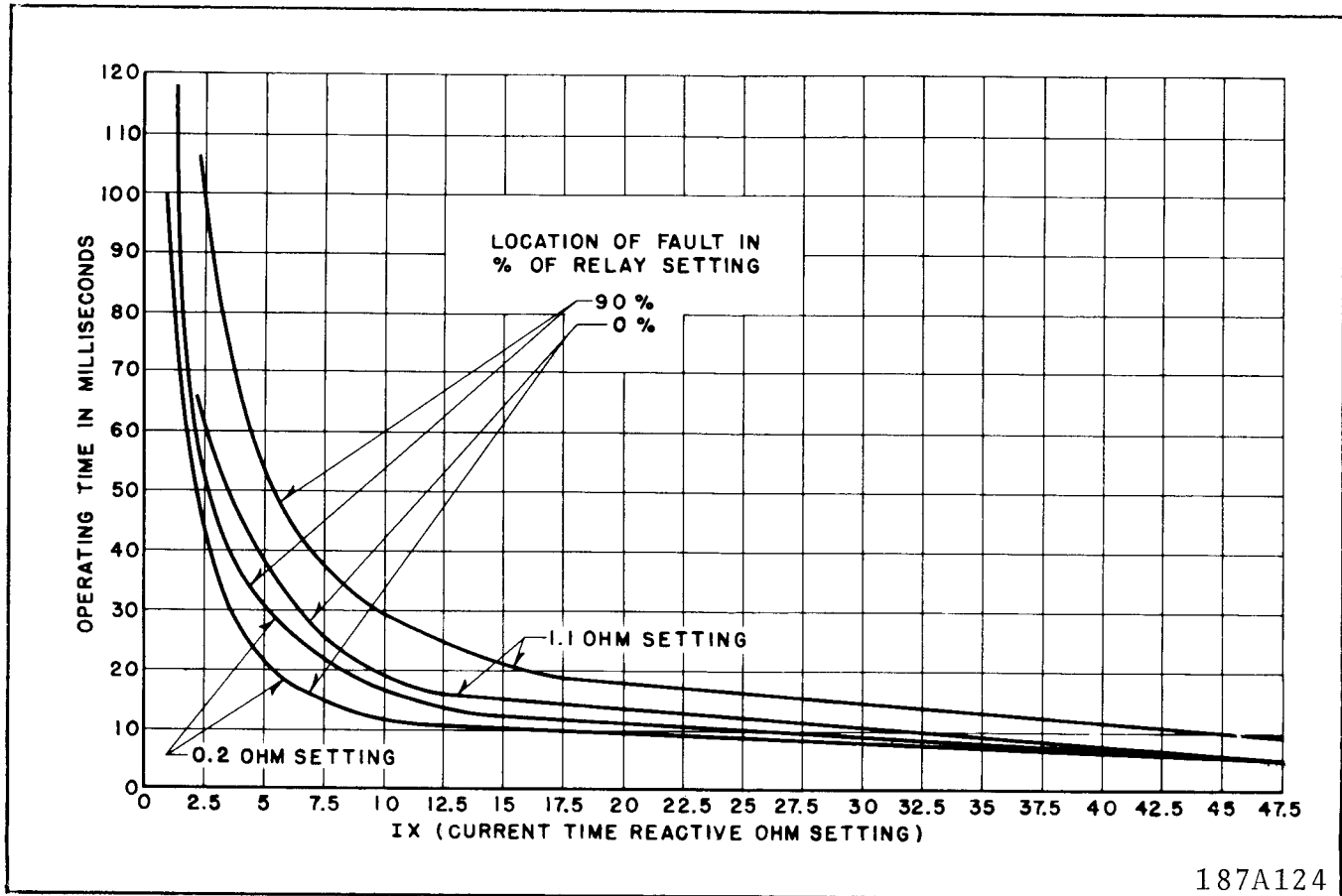
Fig. 16. Typical Operating Time Curves of the Reactance Unit.
