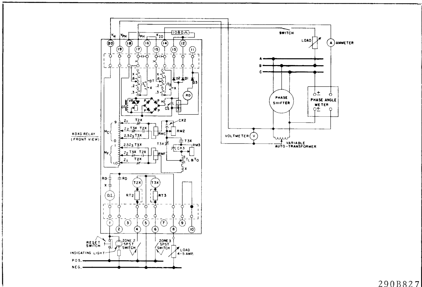
Fig. 13. Test Connections for Type KDXG Relay.
