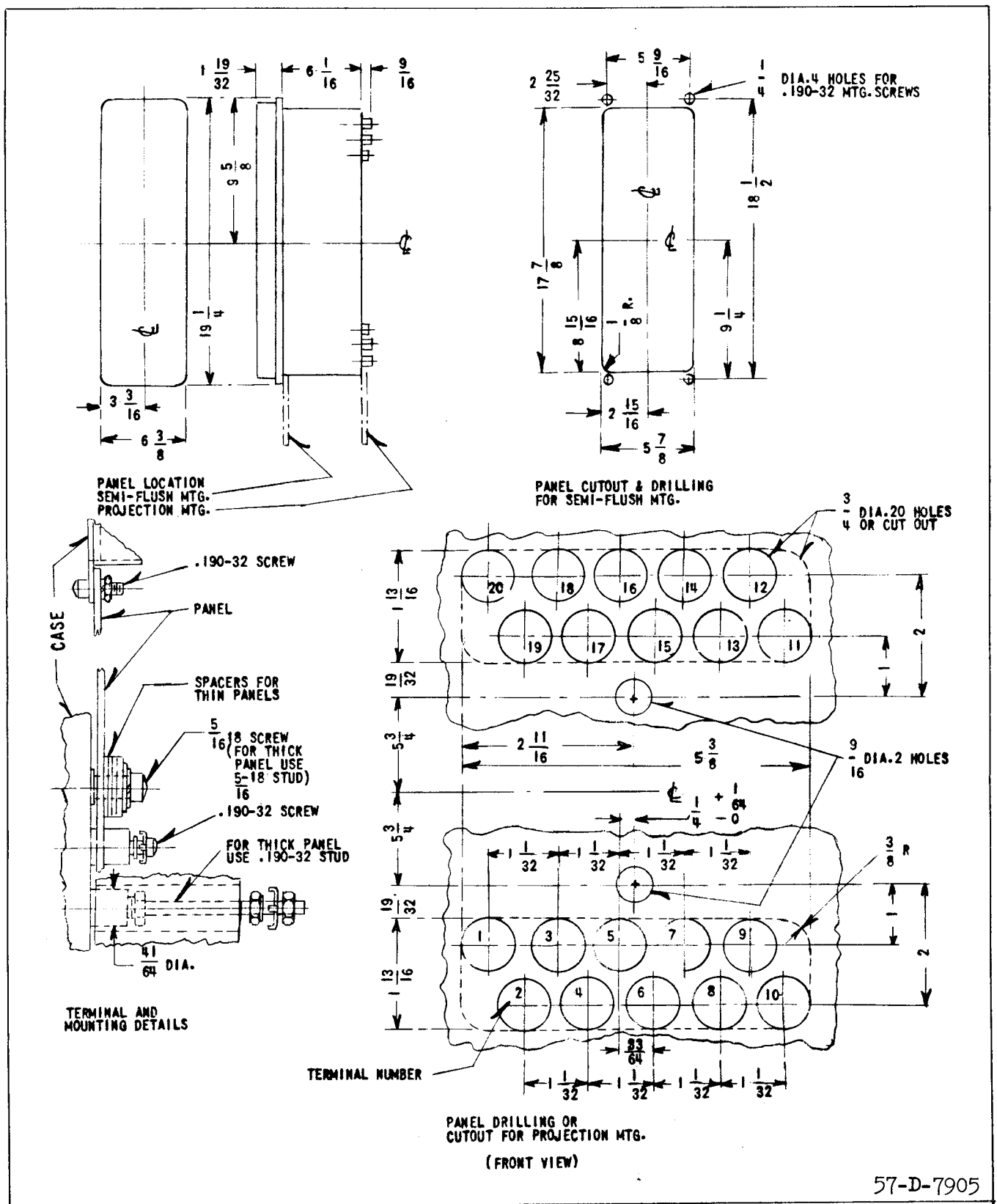
Fig. 16. Outline-Drilling Plan For Type KDXG - Relay in FT42 Case.
