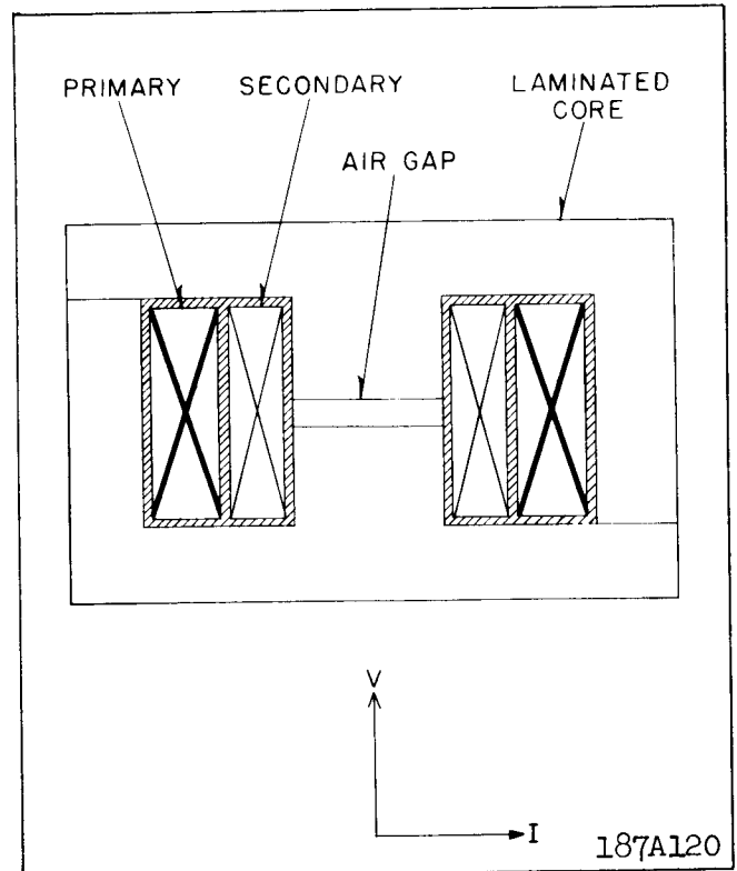
Fig. 3. Compensator Construction.
