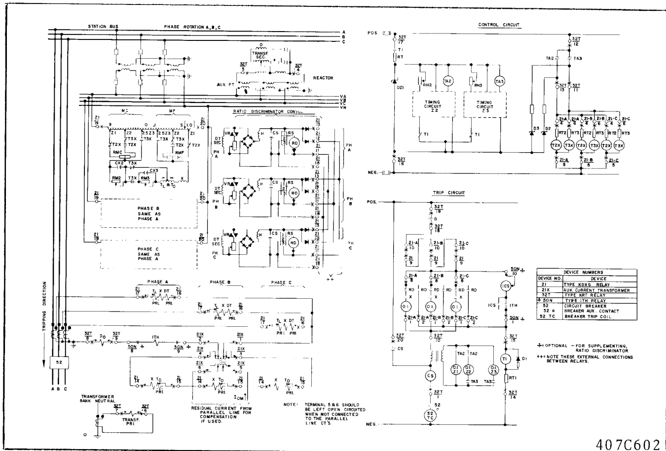
* Fig. 6. External Schematic for Type KDXG Relay with KRT.
