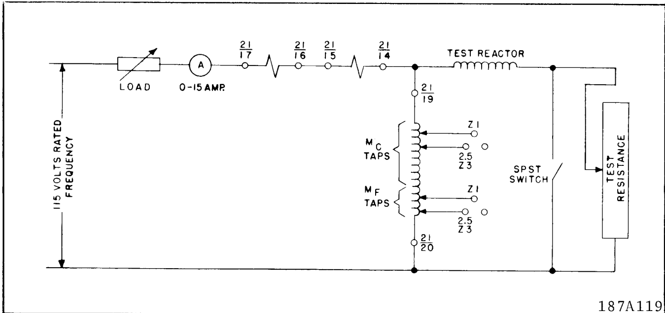
Fig. 15. Circuit for Reactance Unit Phase Angle Adjustment
