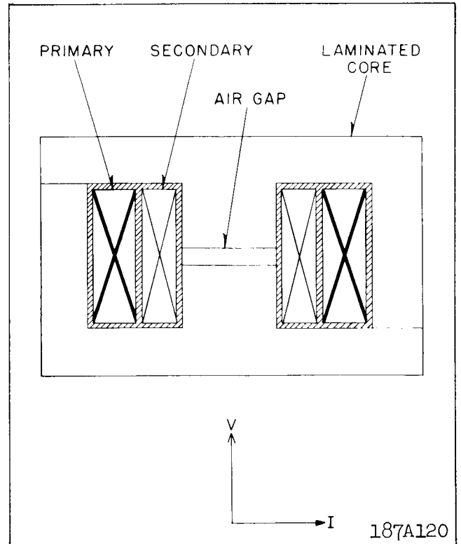
Fig. 3. Compensator Construction.
