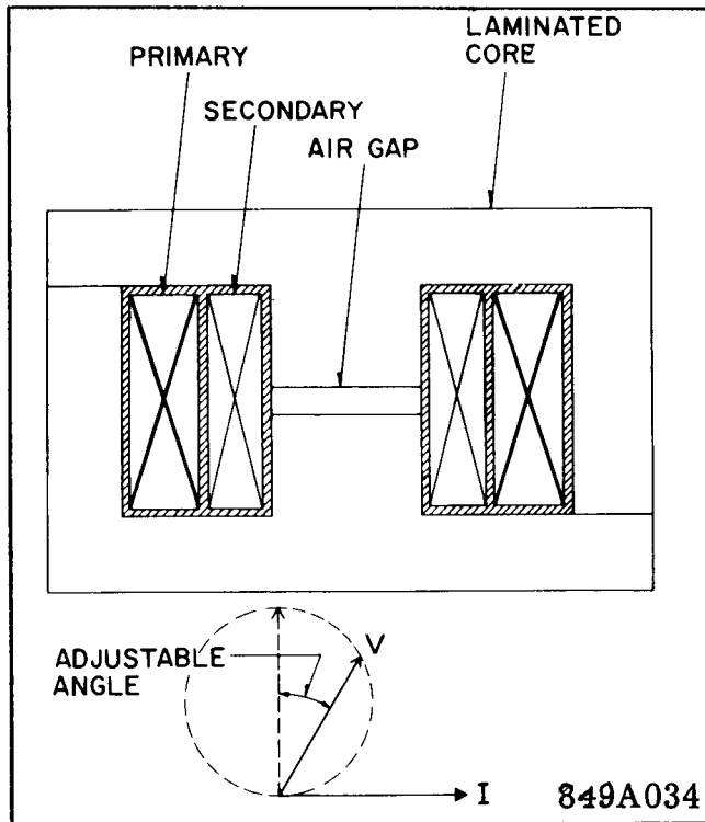
Fig. 2. Compensator Construction
