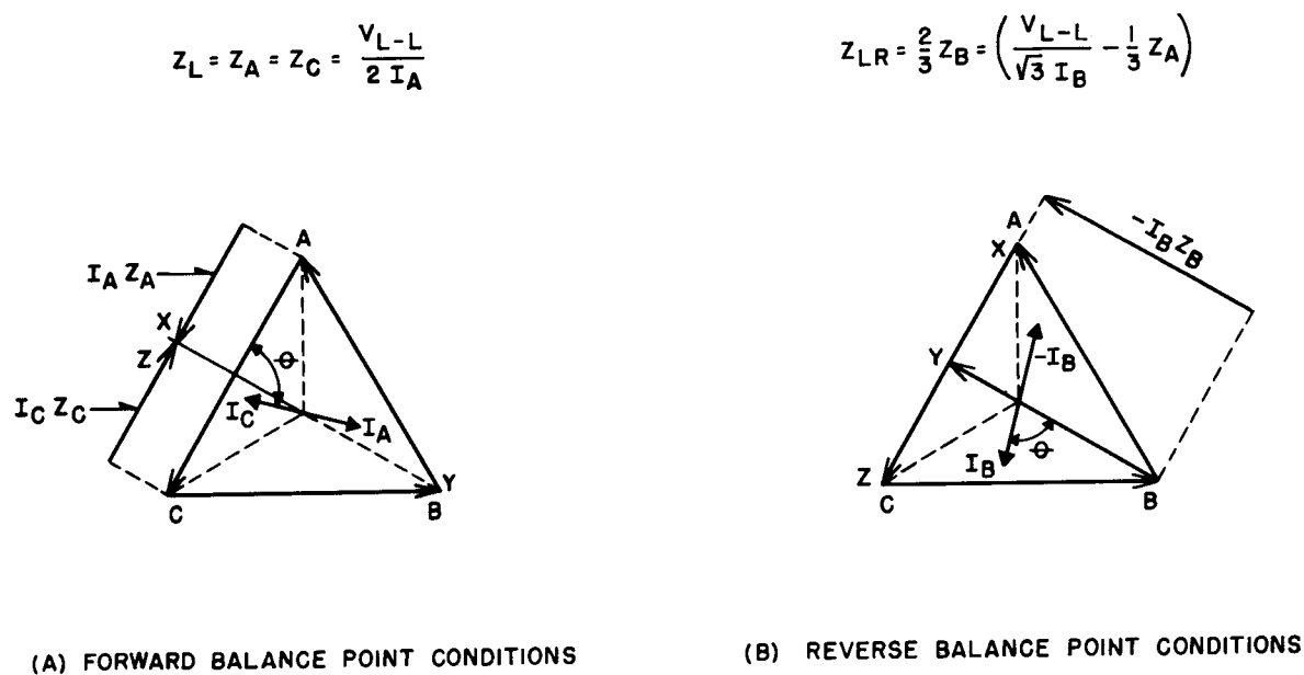
Fig. 9. Vector Diagrams of the Artificial Forward and Reverse Balance Point Conditions when testing with Single Phase Current for Type KS Relay.
