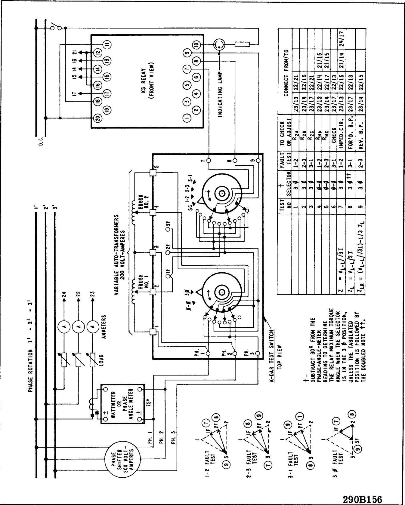
Fig. 7. Test Connections for Type KS Relays.
