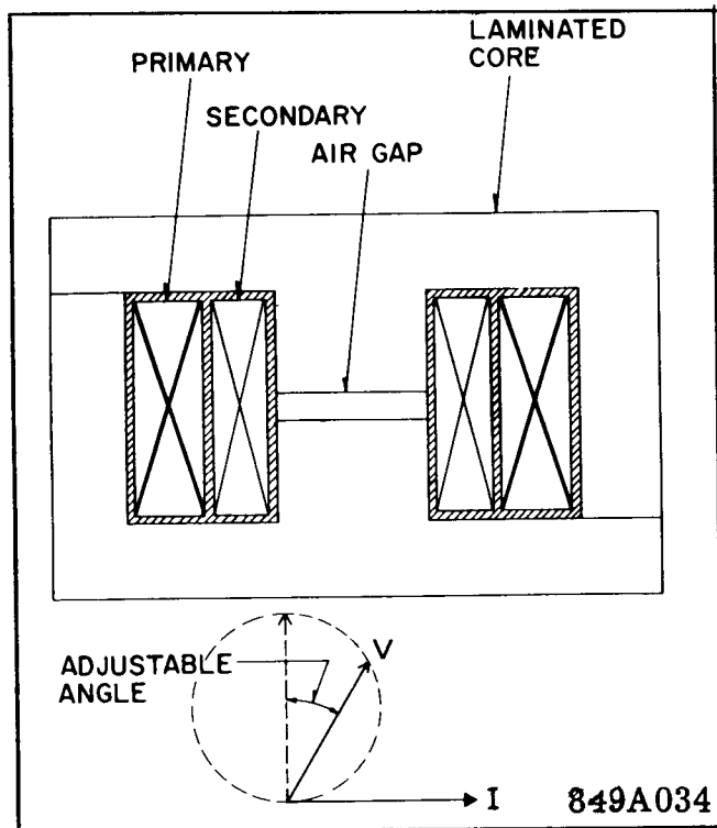
Fig. 2. Compensator Construction
