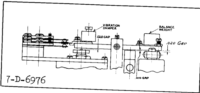
Fig. 1. Sectional View of the Impedance Unit Beam and Contact Assembly.
