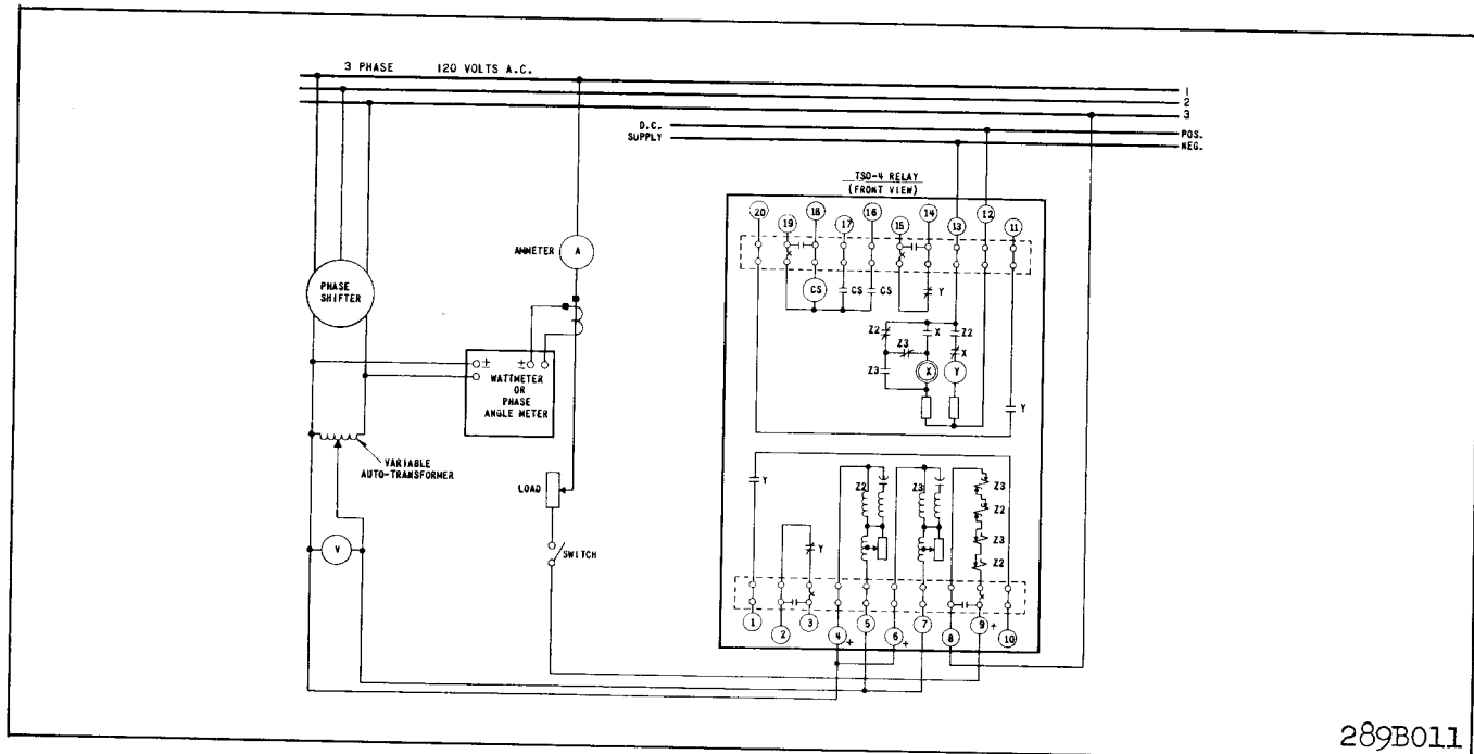
Fig. 6. Diagram of Test Connections for the Type TSO-4 Relay.
