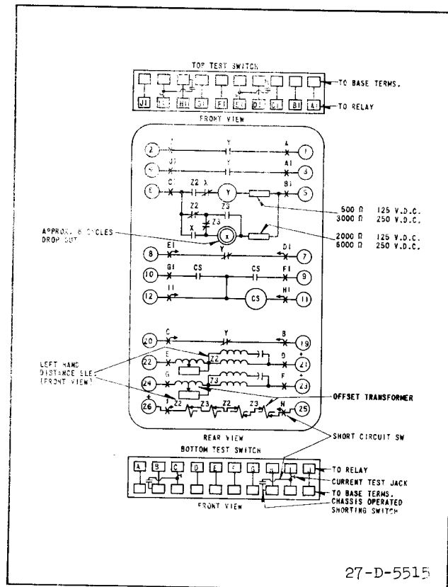
Fig. 2—Internal Schematic of the Type TSO-4 Relay in the Type FT Case. Omit Test Switches for the Relay in the Standard Case.
