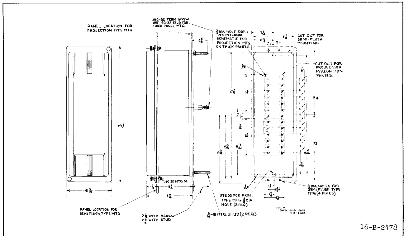
Fig. 8—Outline and Drilling Plan of the M-20 Projection or Semi-flush Type FT Flexitest Case. See the Internal Schematic for the Terminals Supplied. For Reference Only.
