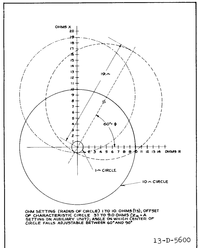
Fig. 3—Operating Characteristics and Range of the Type TSO-4 Relay.
