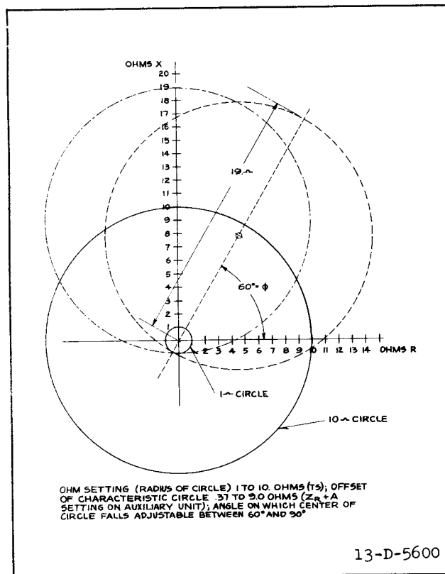
Fig. 3—Operating Characteristics and Range of the Type TSO-4 Relay.
